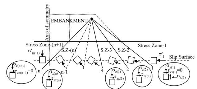
Figure 5. Stress fan and stress-axis rotation beneath the embankment (Öser and Cinicioglu, 2017)
