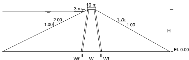
Figure 1. Typical layout of the dam (Djarwadi et al. 2017).
