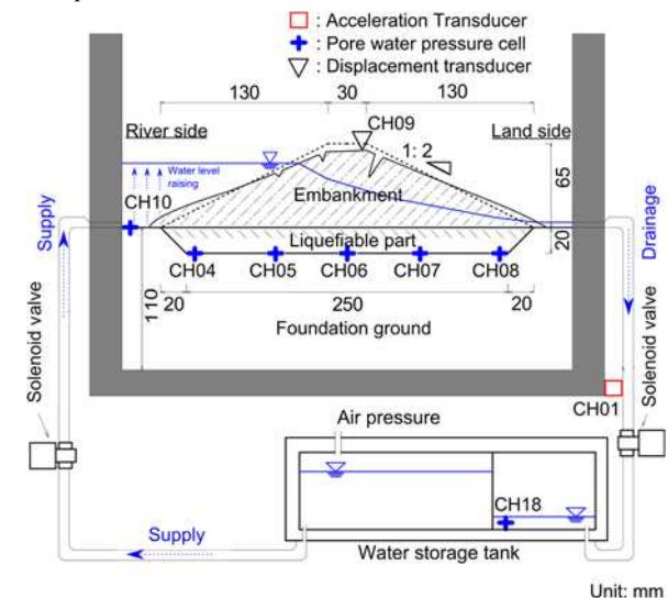
Figure 13. Centrifuge model configuration (Ikami et al. 2017)
