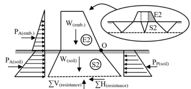
Figure 6. Forces in constituted blocks of the mechanism in the developed limit state method (Öser and Cinicioglu, 2017).
