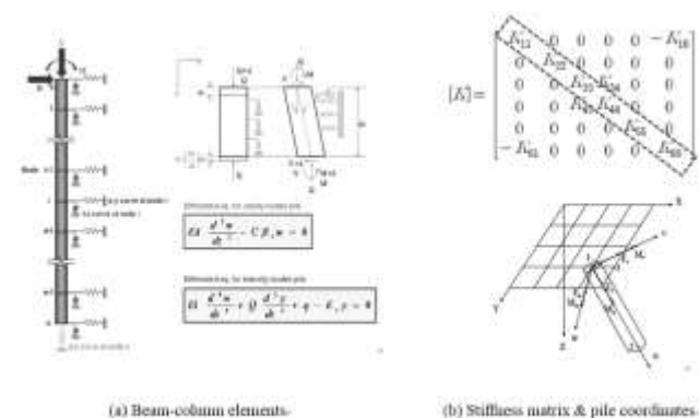
Figure 2. Modeling of pile.
