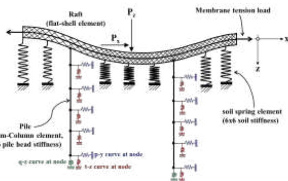
Figure 3. Interactions between raft, piles, and subsoil in present method.
