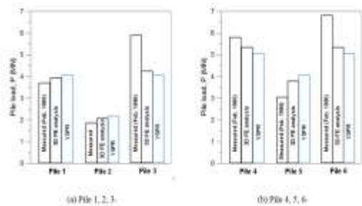
Figure 6. Pile load
