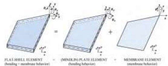
Figure 1. Modeling of flexible raft.
