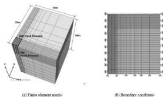
Figure 5. Finite element mesh and boundary condition.
