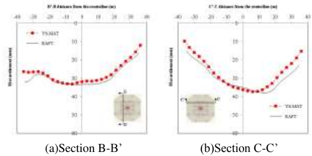
Figure 8. Raft settlement profile
