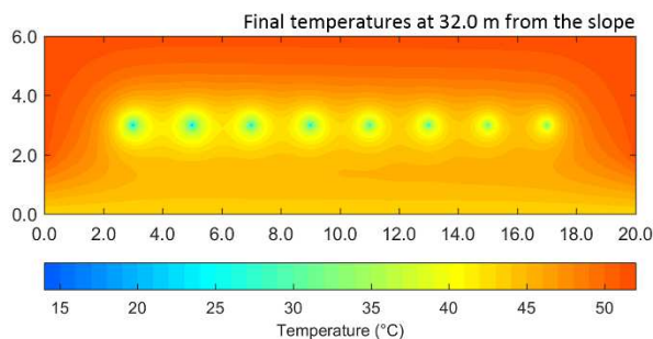
Fig. 7. Finite difference analysis results: 2D temperature profile at 32.0 m from cell slope after 405 h of heat extraction.
