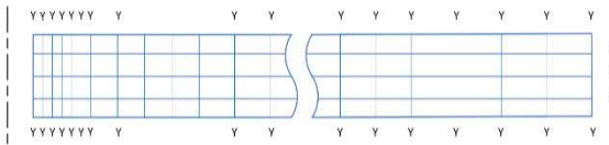
Figure 6. Finite difference axial-symmetric mesh modelled in Flac Software.
