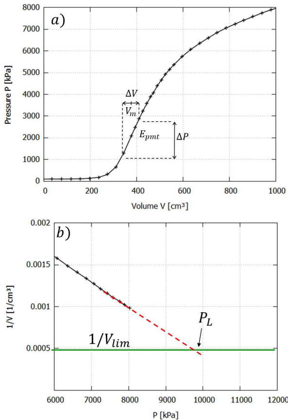
Figure 5. Example of a PMT test and interpretation of a) PMT modulus E_{pmt} and b) PMT pressure limit P_L .
