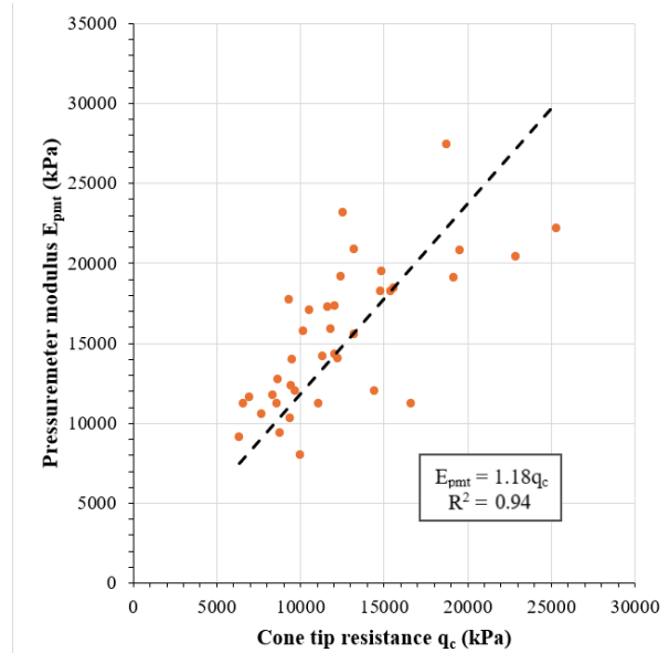
Figure 7. Relationship between cone tip resistance ( q_c ) and pressuremeter modulus E_{pmt} for all data from site 1 and compared with literature relationship
