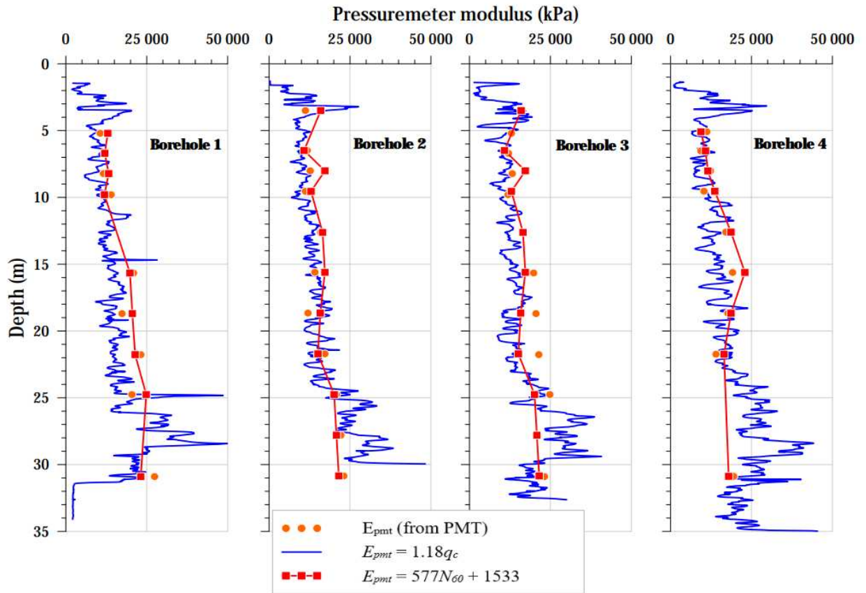
Figure 9. Comparison between the pressuremeter modulus ( E_{pmt} ) from PMT tests, from CPT i.e. 1.18q_c and from the SPT- N_{60} present relationships studied, for the boreholes at site 1.
