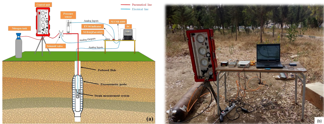
Figure 10. (a) Schematic sketch of the pressuremeter equipment on site assembly; (b) Assembly and overview on site.
