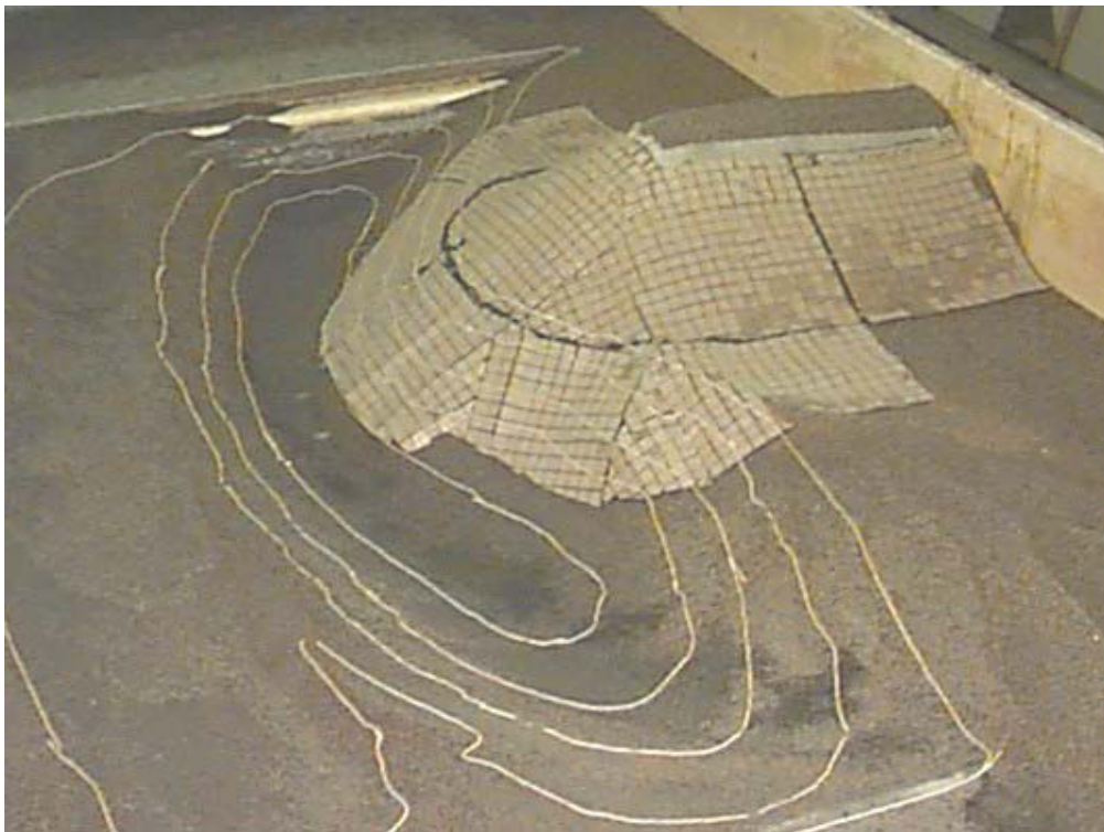
Figure 11 – Typical scour hole development for cable-tied block protection (Test 5), viewed from downstream. In this test, the protection was deemed not to have failed
