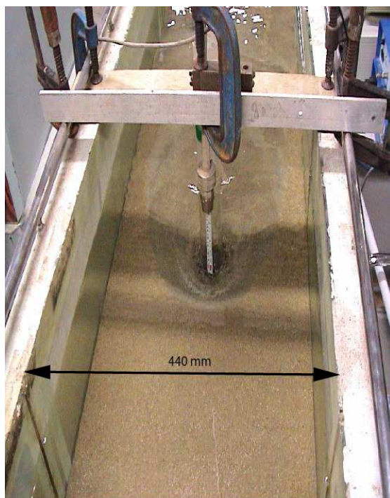
Figure 2. Photograph of the flume and test structure used in these tests. The flume is located in the Hydraulics Laboratory at the University of Auckland in Auckland, New Zealand.
