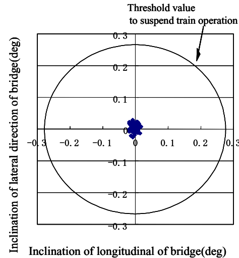
Fig.5 Scattered diagram of the inclinations of a certain bridge pier
