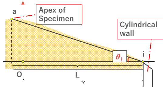
Figure. 8 Definition of angle of repose
