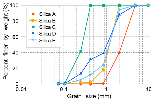
Figure 6 Grain size distribution
