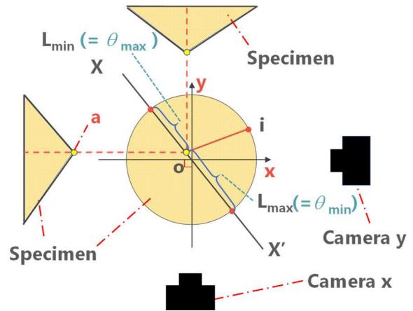
Figure. 7 Schematic diagram for identification of apex by two images and for setting of angle of repose, \theta_i
