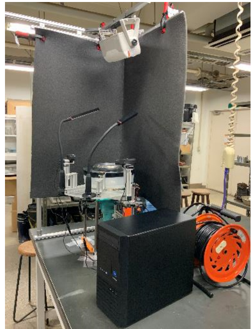
Figure. 1 External view of the experimental apparatus
