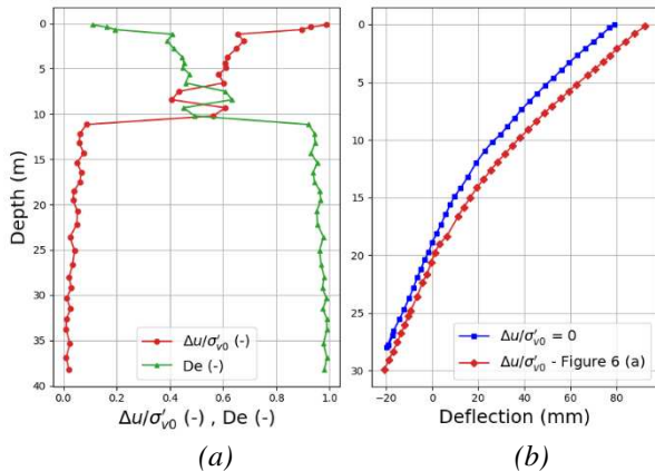
Figure 6. (a) Excess pore pressure ratio and shear strength degradation factor ( De ) depth profiles. (b) Monopile lateral deflection using p - y soil reaction curves.
