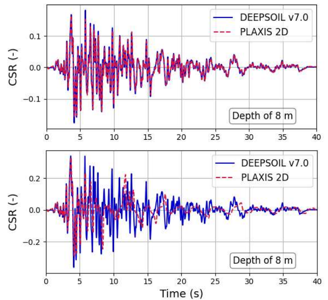
Figure 3 CSR time histories at 8 m depth, computed using PLAXIS 2D and DEEPSOIL v7.0. The top and bottom
