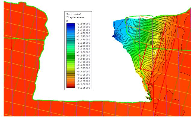
Figure 7. Horizontal displacement field in the asymmetric plane-strain model without application of the circumferential confinement correction (failure of the right slope, T1 tomb).
