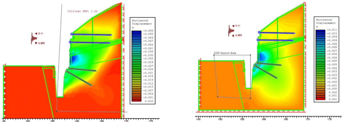
Figure 12. Left: Seismic 2D elasto-plastic analysis using the SSR method (finite elements) – stabilization measures – downward vertical acceleration component – F_{s,min} = 1.22 . Right: Seismic 2D elasto-plastic stability analysis of the stabilization measures with finite elements – downward vertical acceleration component – maximum permanent horizontal displacement \Delta h = 0.011 m (Geo.Per. S.A., 2021).
