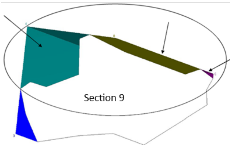
Figure 3. Wedges susceptible to failure near Section 9 of Dikteon Cave (unsupported condition). 0.0 \leq FS_{min, Static Load} \leq 1.2 and 0.0 \leq FS_{min, EQ} = 0.9 .
