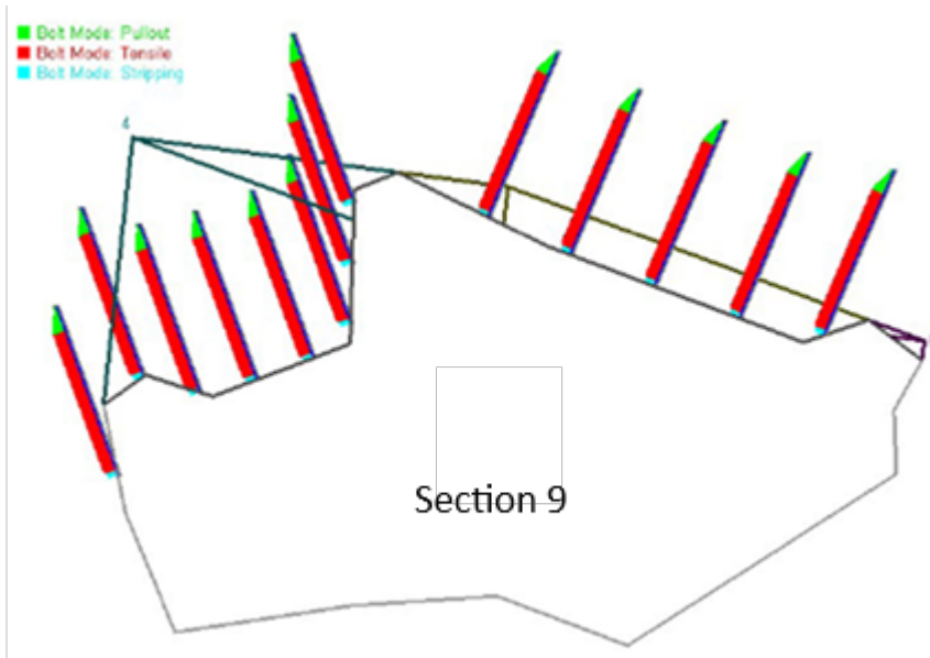
Figure 4. Wedges susceptible to failure near Section 9 of Dikteon Cave (stabilisation measures). FS_{min, Static Load} = 1.78 , FS_{min, EQ} = 1.12 .
