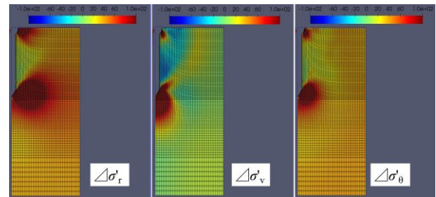
(a) Case 3: small width (140 mm)
