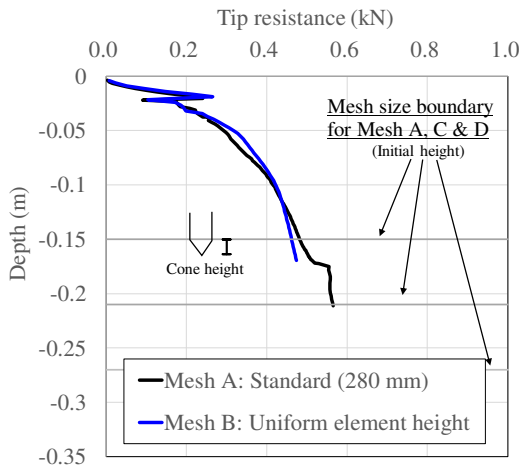
Figure 5. Confirmations of the extent of influence of element size at the cone apex on the tip resistance.
