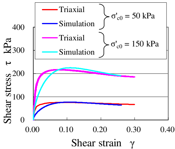
Figure 4. Examples of the element responses of SYS Cam clay model by using the material properties shown in Tables 2 and 3.
