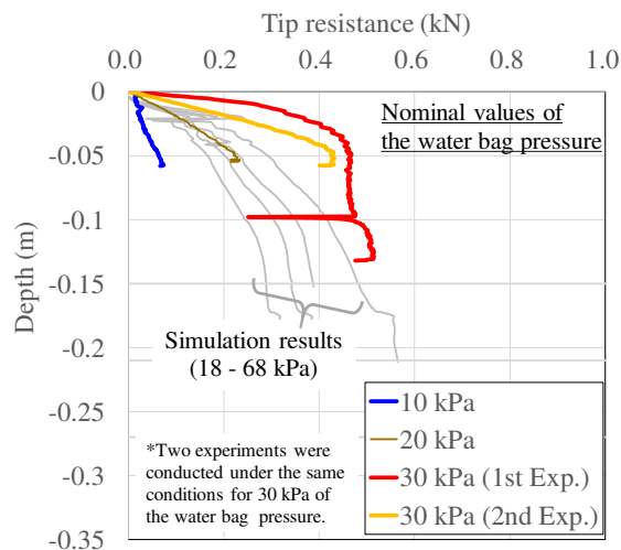
Figure 12. Comparisons of all the results obtained from both experiment and numerical simulations conducted at different over burden pressures.
