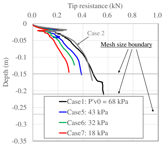
Figure 9. Confirmations of the realization of the relationships between the overburden pressure and the tip resistance.
