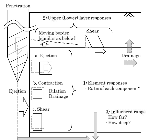
Figure 1. Penetration mechanisms; the logic solving it as a boundary value problem.
