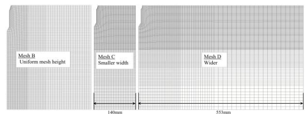
(b) Other models
