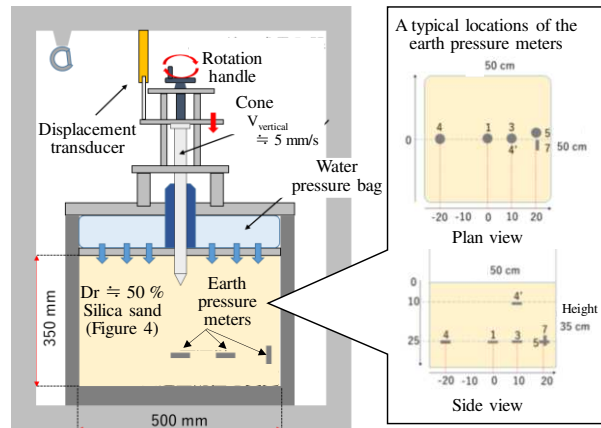
Figure 10. Outlines of a preliminary calibration chamber test.
