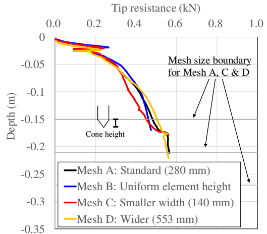
Figure 7. Confirmations of the extent of influence of element size at the cone apex on the tip resistance with using models having different width.
