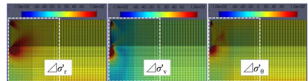
(b) Case 4: wider model (553 mm)
