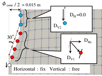
Figure 3. Calculated procedures of cone penetration.
