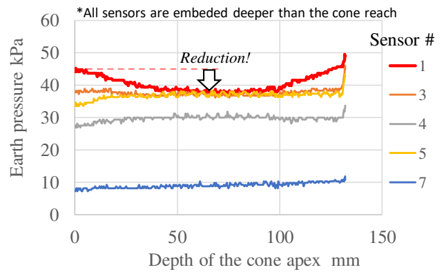
Figure 11. A typical measurement result of earth pressures.
