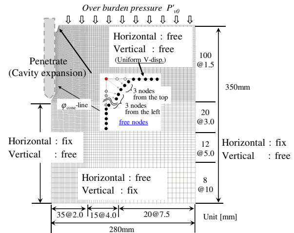
(a) Standard model (Mesh A)
