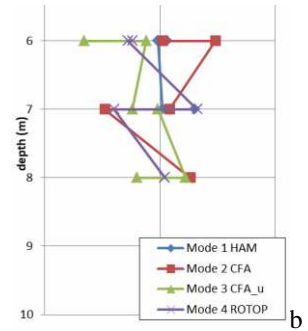
Figure 10. Influence of the mode of placement on the on the limit pressure and pressuremeter modulus for an alluvial sand at Honfleur
