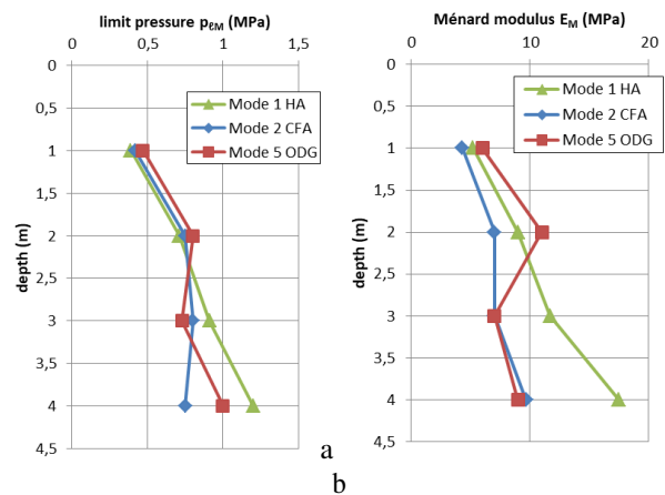
Figure 8. Influence of the mode of placement on the on the limit pressure and pressuremeter modulus for a silt of Mont Gaillard
