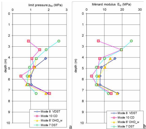
Figure 12. Influence of the mode of placement on the on the limit pressure and pressuremeter modulus for a chalk close to Rouen
