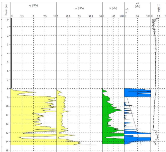
Figure 5. Measurements with a static penetrometer : q_c , f_s , u_2 , angle
