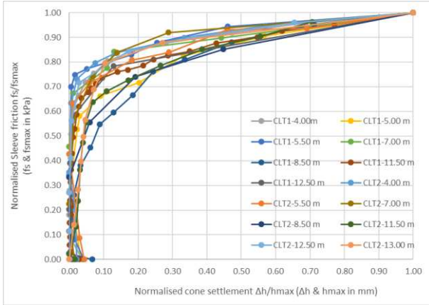
Figure 18. CLT Tests for SARRIANS Site: f_s
