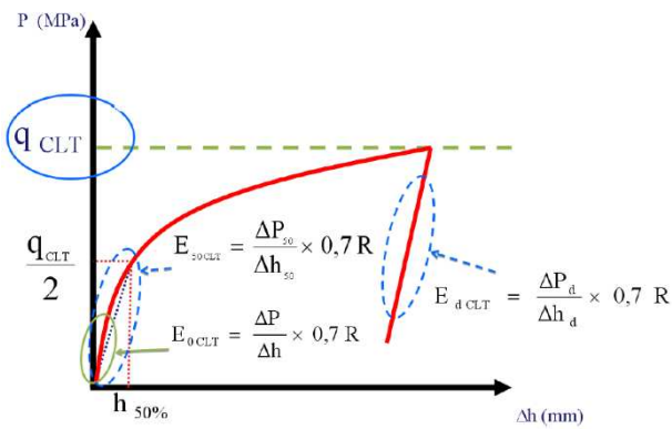
Figure 2. Determination of deformation modulus E_{0,CLT} , E_{50,CLT} and E_{d,CLT} according to the pressure versus deformation curve (after Ali., 2011 [1])
