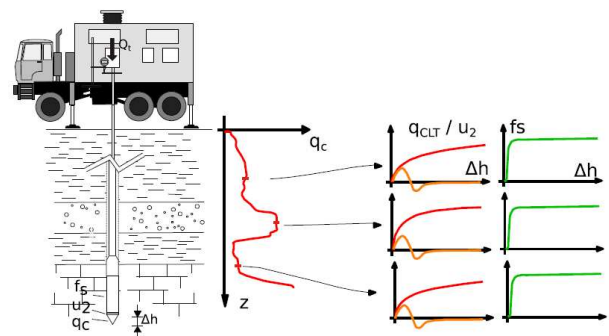
Figure 1. Cone Loading Test principles (Reiffsteck., 2017 [2])
