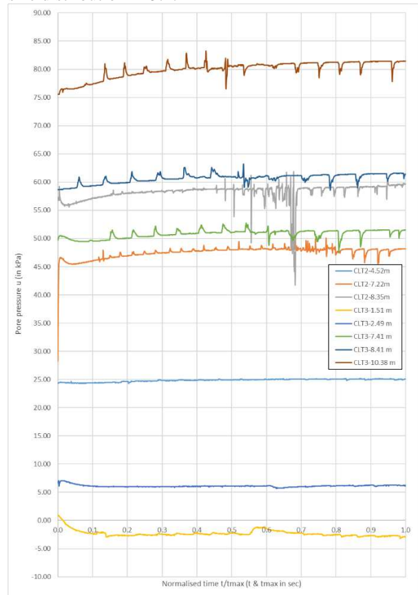
Figure 22. Pore pressure u_2 (kPa) during CLT Tests in SETE Site
