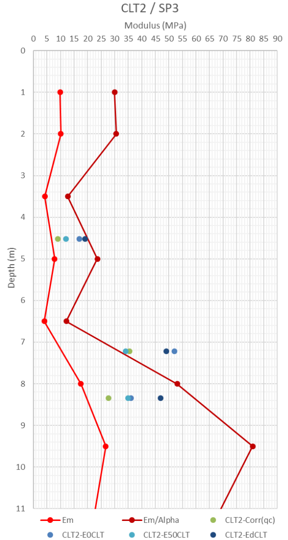
Figure 20. E_{0CLT} comparison with E_M , E_M/\alpha and Young modulus obtained by CPT correlation, for SETE site (CLT2)
