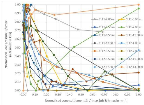
Figure 19. CLT Tests for SARRIANS Site: u_2
