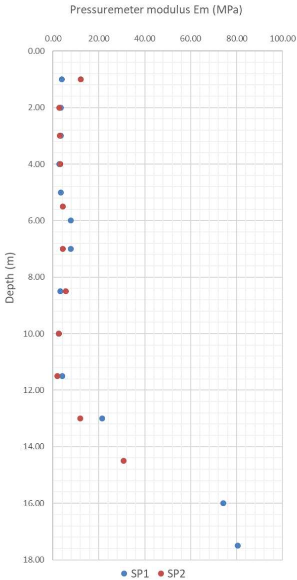
Figure 11. Ménard pressuremeter modulus ( E_M ) measures for SARRIANS site
