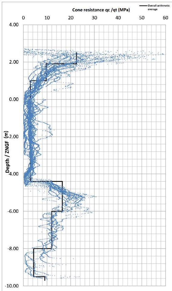
Figure 8. Cone resistance ( q_c/q_t ) measures for SETE site
