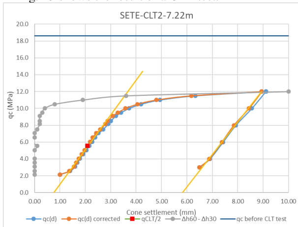
Figure 13. Example of a CLT test interpretation – SETE-CLT2-7.22m
