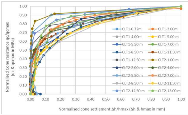
Figure 17. CLT Tests for SARRIANS Site: q_c
