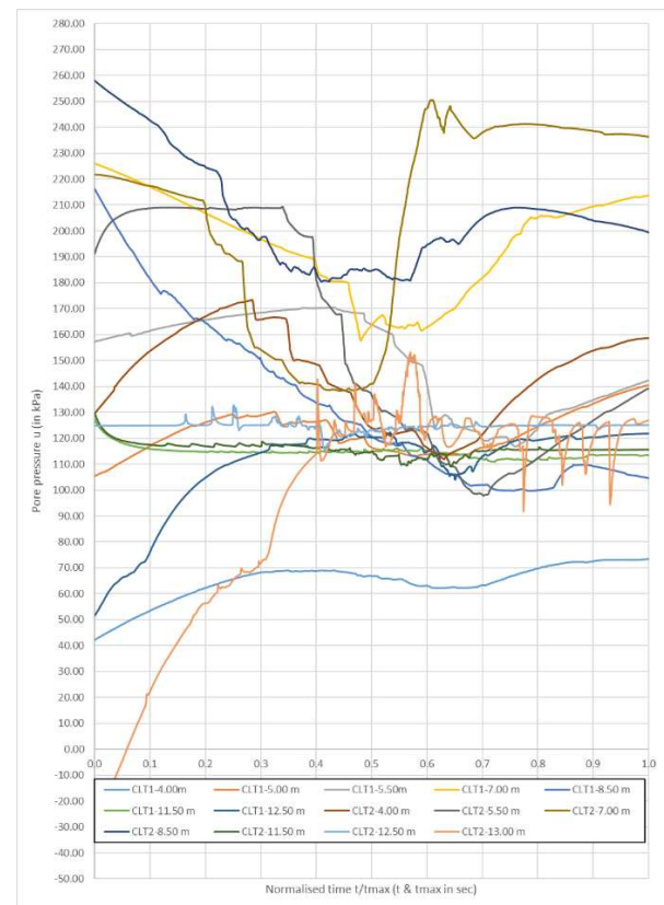
Figure 23. Pore pressure u_2 (kPa) during CLT in SARRIANS Site
