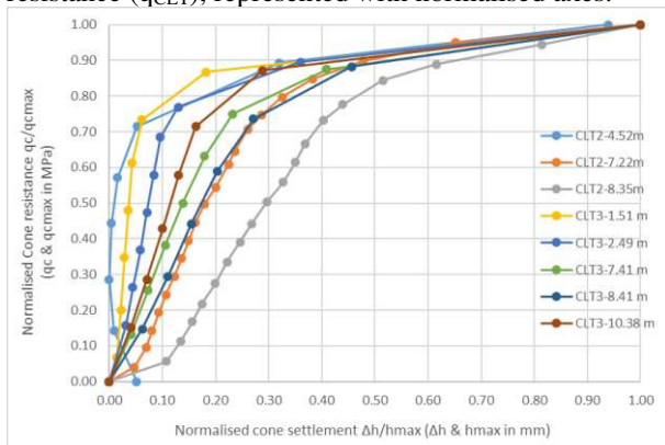
Figure 14. CLT Tests for SETE Site: q_c
