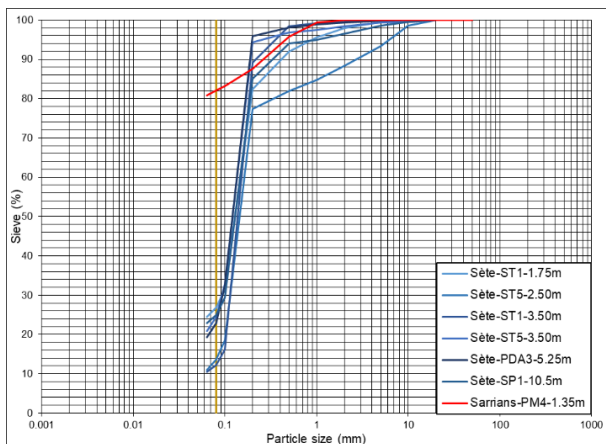
Figure 12. Particle size distributions for SETE and SARRIANS soils
