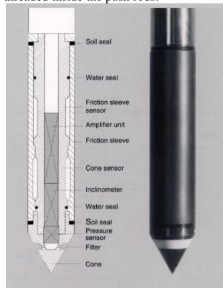
Figure 4. The penetrometer cone
