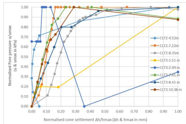
Figure 16. CLT Tests for SETE Site: u_2
