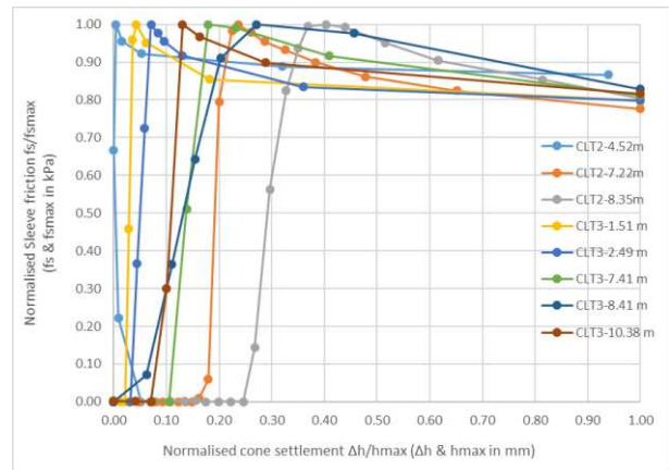
Figure 15. CLT Tests for SETE Site: f_s
