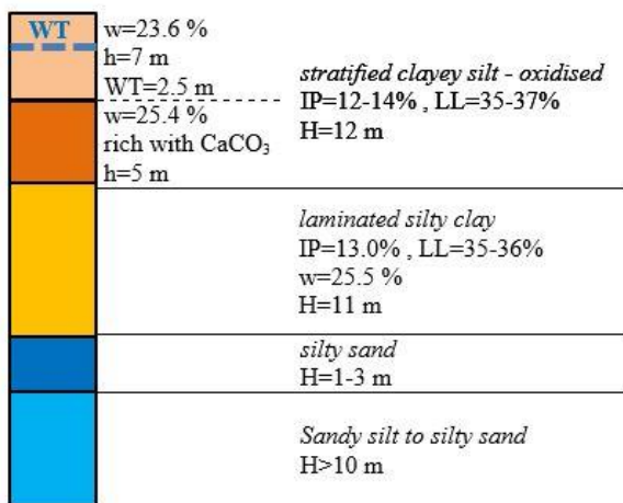
Figure 2. Soil profile at Kuzmin test site
