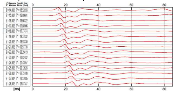
Figure 7. SPDMT recorded seismic traces of P-wave at Kuzmin test site
