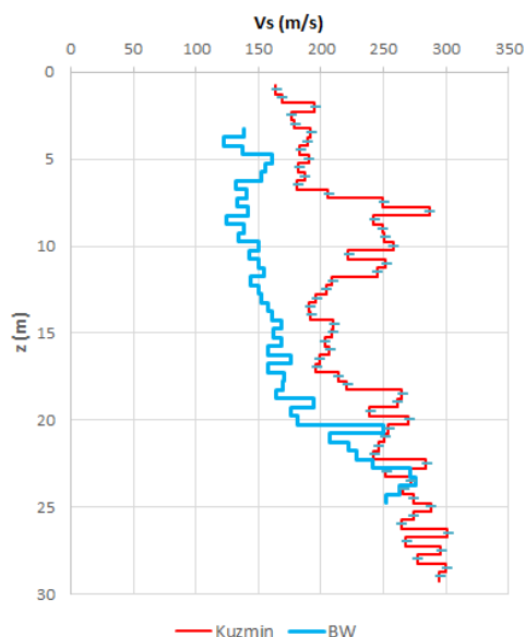
Figure 10. V_s profiles measured with SPDMT
