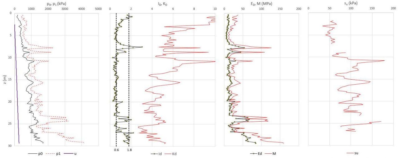
Figure 5. DMT results at Kuzmin test site
