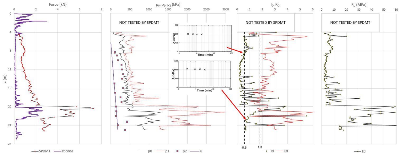
Figure 4. DMT results at BW test site
