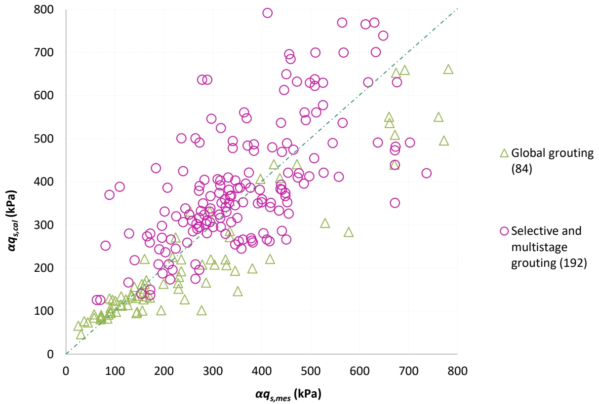
Figure 5. Comparison of measured and calculated shaft friction, respectively \alpha q_{s,mes} and \alpha q_{s,cal} (by execution conditions – 276 q_s measurements)
