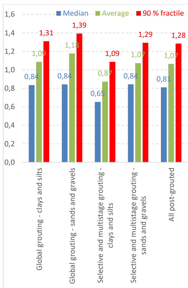
Figure 8. Average, median and 90 % fractile for clays and silts then sands and gravels
