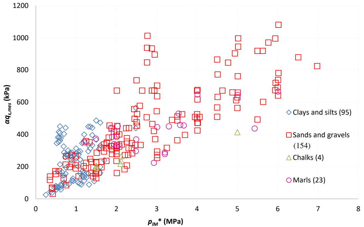
Figure 2. Obtained results (by ground types – 276 q_s measurements)
