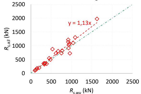
Figure 1. Comparison of failure criteria
