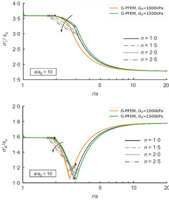
Figure 3. Comparison of numerical (G-PFEM) and analytical [12] results in terms of normalized effective radial ( \sigma'_r/s_u ) and circumferential ( \sigma'_c/s_u ) stresses over normalized radius.
