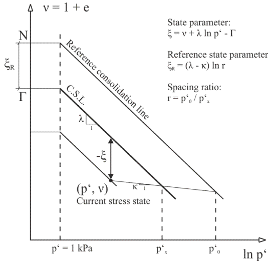
Figure 1. Representation of state parameter and critical state constants according to [8].
