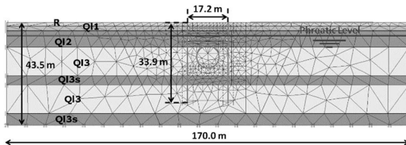
Figure 4. Finite element mesh.
