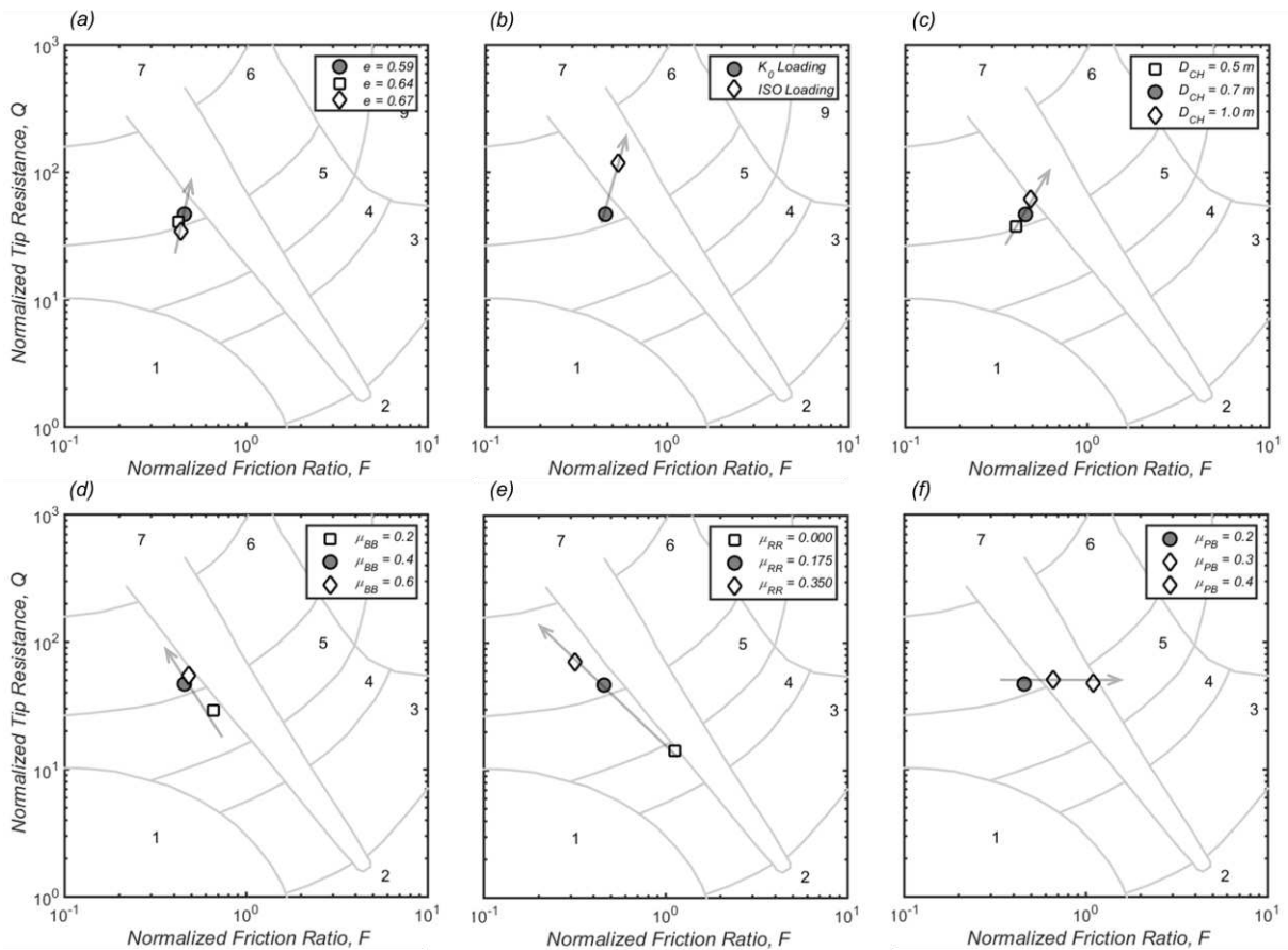
Figure 9. Normalized CPT soil behavior type classification of simulations with varying (a) void ratio, (b) boundary conditions, (c) chamber diameter, (d) inter-particle friction coefficient, (e) rolling resistance coefficient and (f) varying probe-particle friction coefficient.
