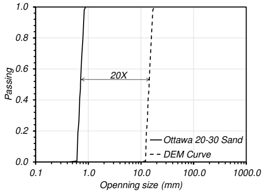
Figure 2. Simulated grain size distribution.
