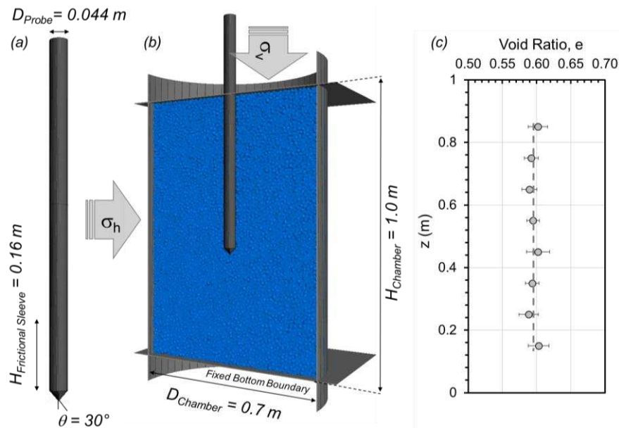
Figure 1. Simulated (a) CPT probe and (b) Virtual Calibration Chamber (VCC), and (c) local void ratio distribution along VCC height (note: error bars show standard deviation in void ratio).
