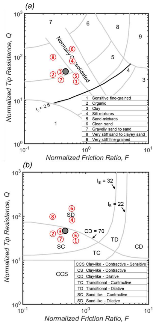
Figure 4. Results from baseline simulation plotted on (a) Robertson (1990) and (b) Robertson (2016) CPT-based soil classification charts.
