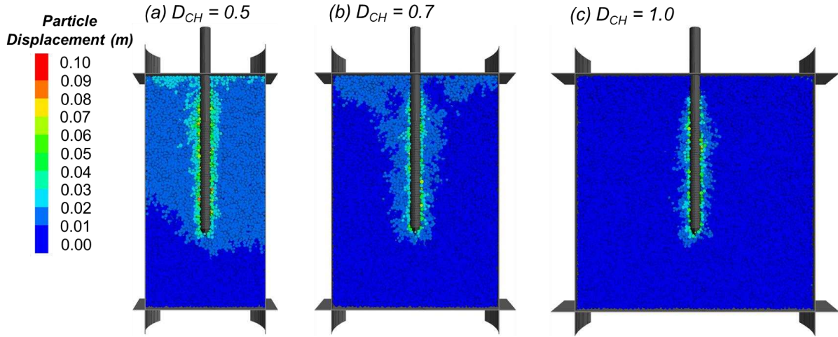
Figure 6. Particle displacements along vertical cross sections for simulations on VCCs of different diameter Note: all measurements taken at a CPT penetration depth of 60 cm.
