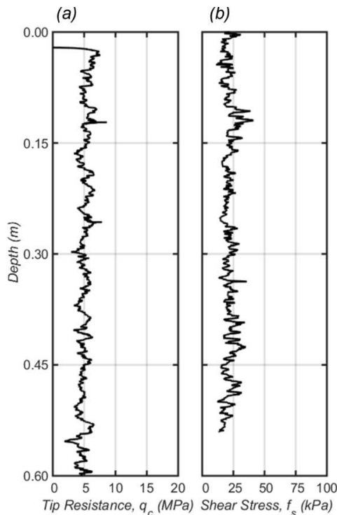
Figure 3. Profiles of (a) q_c and (b) f_s for baseline simulation.
