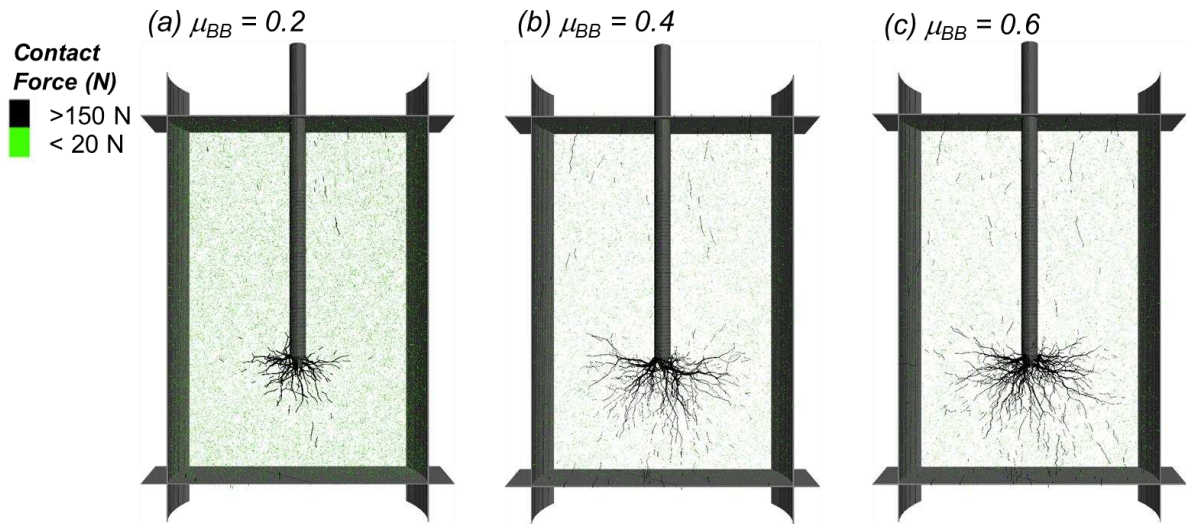
Figure 8. Force chain maps along vertical cross section for simulations with inter-particle friction coefficients of (a) 0.2, (b) 0.4, and (c) 0.6. Note: all measurements taken at a CPT penetration depth of 60 cm.
