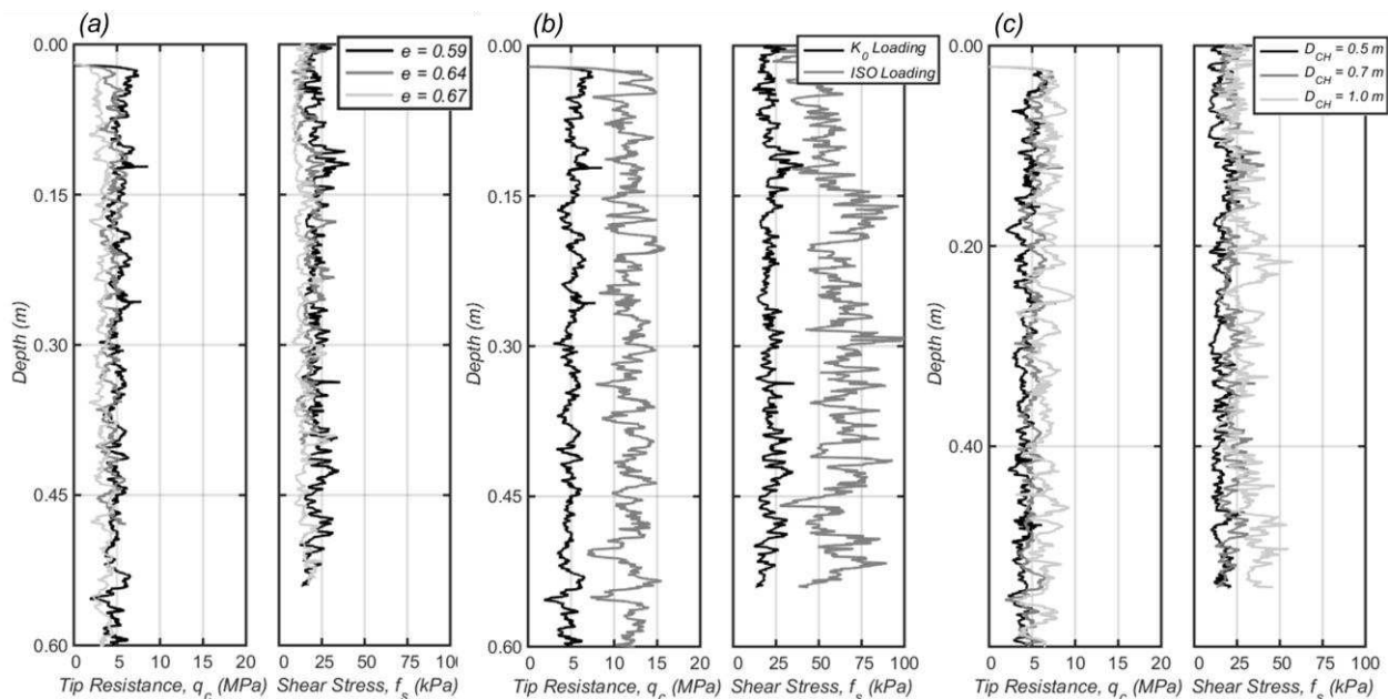
Figure 5. Profiles of (a) q_c and (b) f_s for simulations with varying (a) void ratio, e , (b) stress boundary conditions, and (c) chamber diameter, D_{CH} .
