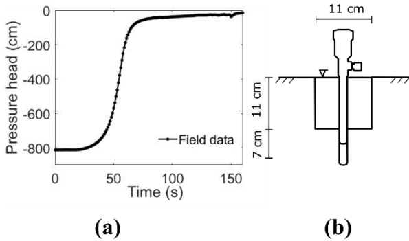
Figure 8. MItest measurement on a residual soil test site whose unsaturated hydraulic parameters are unknown (a) MItest response (b) MItest field specifications
