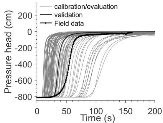
Figure 9. Prediction of 100 pressure head curves for 200 seconds time-lapse.
