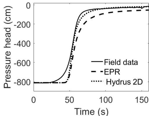
Figure 10. Graphical results of inversion for field data.
