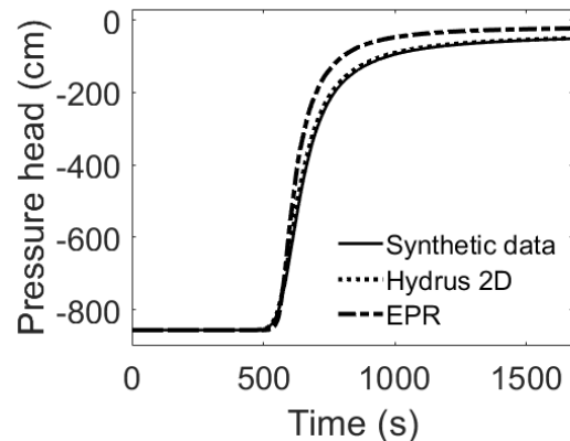
Figure 7. Graphical results of inverse analyses for synthetic data.
