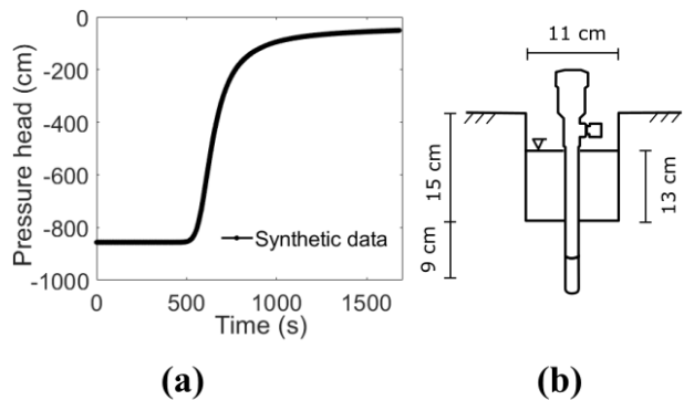
Figure 5. Synthetic data whose unsaturated hydraulic parameters are known. (a) Mltest response. (b) Mltest field specifications.
