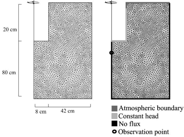
Figure 2. Numerical settings: type and size of geometry, element sizes and boundary condition (Out of scale).
