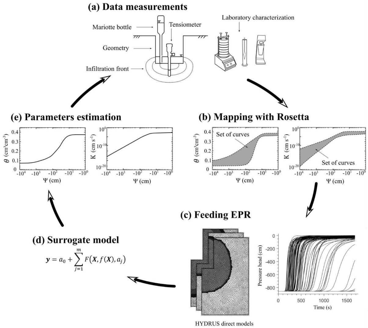
Figure 1. Methodology used to calibrate a surrogate model with the monitored infiltration test. (a) Data collection through field and laboratory measurements; (b) Parameters mapping through laboratory results and Rosetta prediction; (c) A series of forward models to generate a predetermined number of pressure head versus time curves; (d) The EPR algorithm uses the synthetic curves to calibrate a model; (e) Parameters estimation through inverse modelling.
