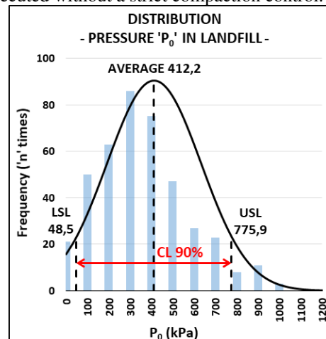
Figure 12. P_0 distribution in the landfill without compaction control.
