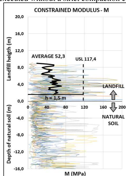
Figure 18. M overlap in the landfill without compaction control.
