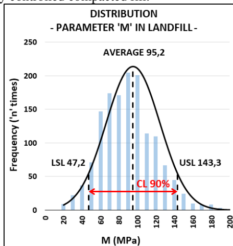
Figure 14. M distribution in the rigorously controlled landfill.
