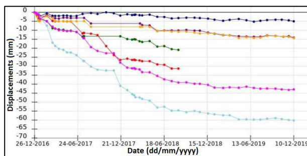
Figure 21. Settlements measured by geotechnical instrumentation.
