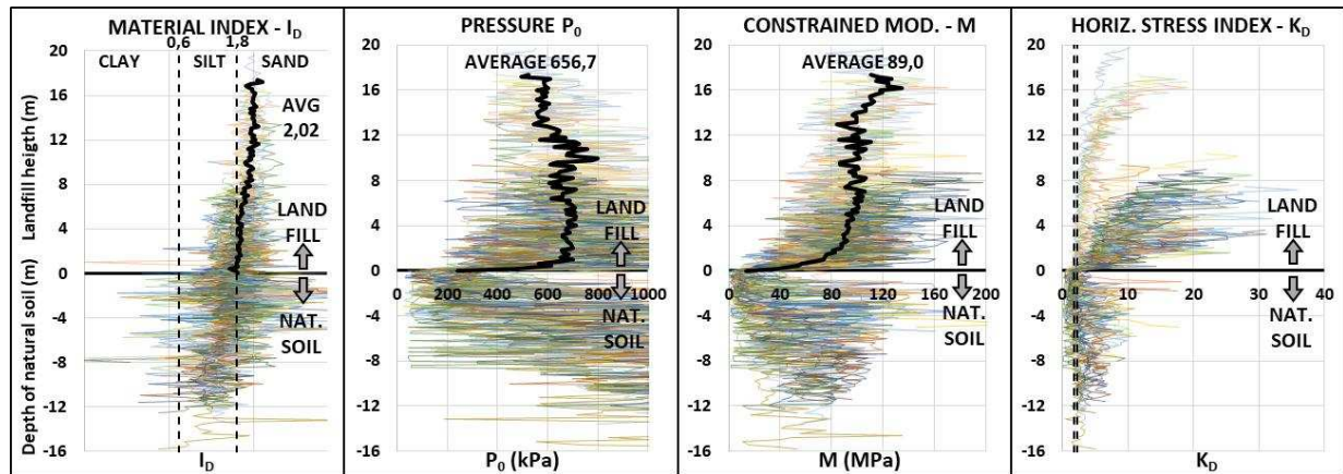
Figure 10. Results overlap of all DMT tests.
