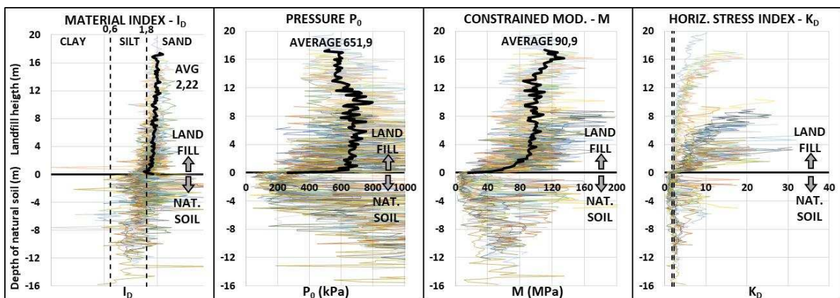
Figure 9. Results of tests that indicated material index of sand in landfill.
