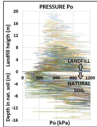
Figure 7. P_0 results overlap (approximately 50 different tests).
