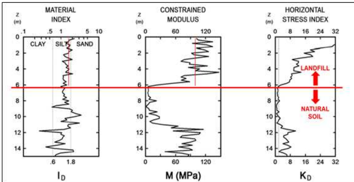
Figure 5. Example of a DMT result (DMT-308), indicating the transition from landfill to natural soil.
