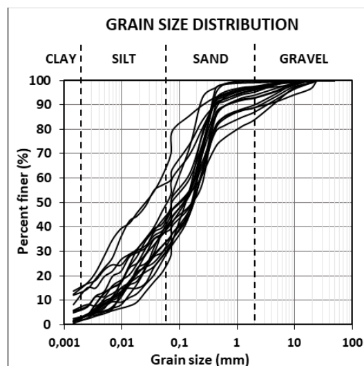
Figure 2. Grain size distribution of soil sampling executed in landfill.
