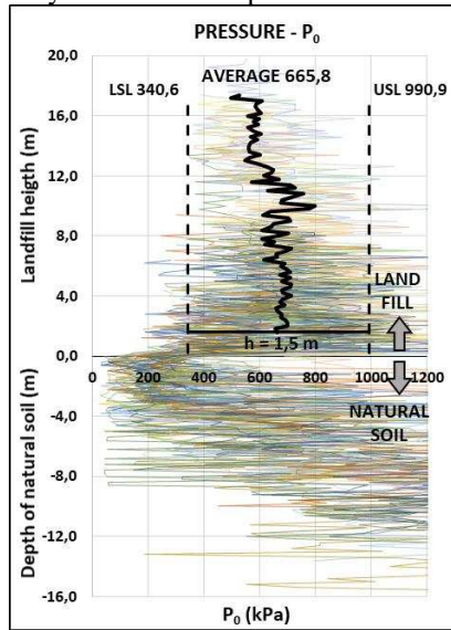
Figure 13. P_0 overlap in the rigorously controlled landfill.
