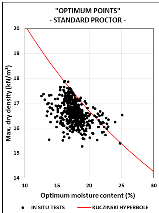
Figure 3. Dispersion of the “optimum points” obtained in the tests.
