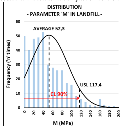
Figure 17. M distribution in the landfill without compaction control.
