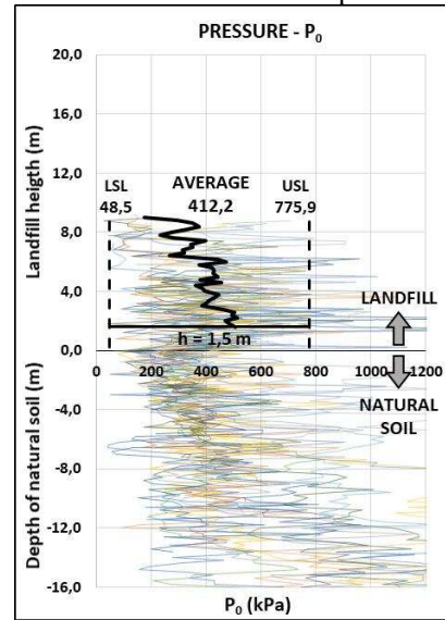
Figure 16. P_0 overlap in the landfill without compaction control.
