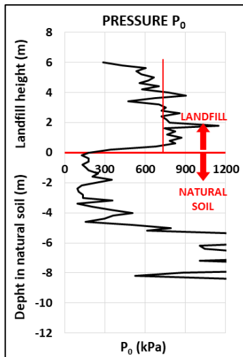
Figure 6. Results of P_0 in the DMT-308.
