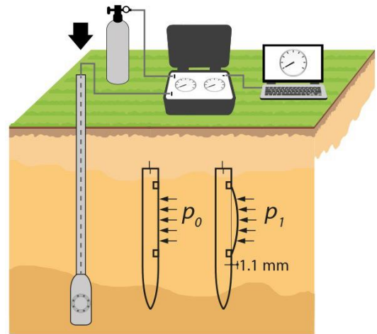
Figure 4. Schematic representation of the dilatometer test.
