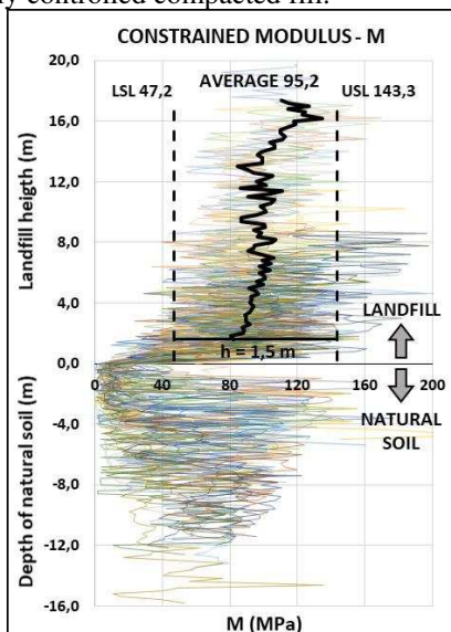
Figure 15. M overlap in the rigorously controlled landfill.
