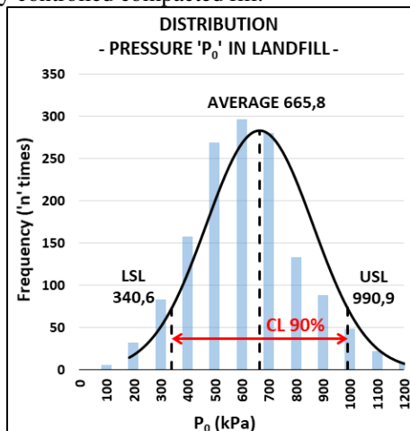
Figure 11. P_0 distribution in the rigorously controlled landfill.
