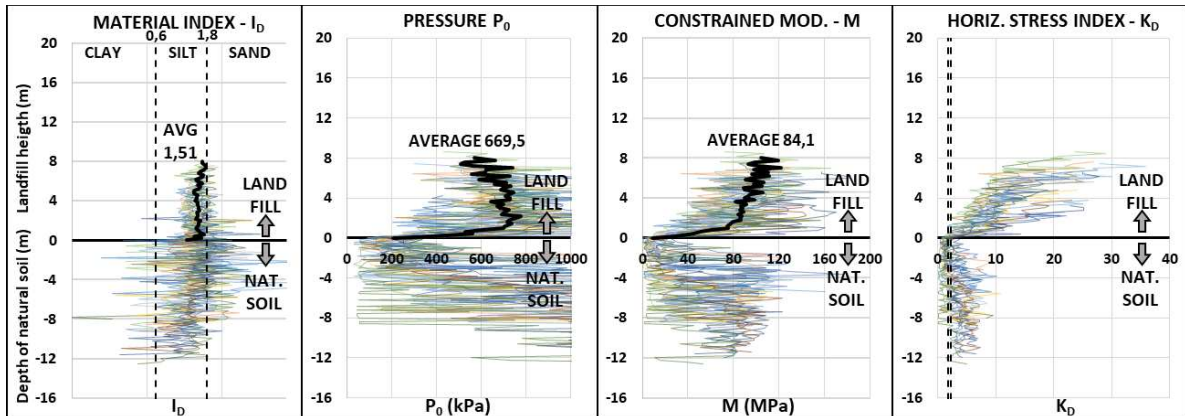
Figure 8. Results of tests that indicated material index of silt in landfill.
