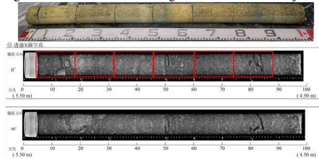
Figure 5. X-ray photograph of undisturbed gravel soil (Chubu Resion site: Red line shows the cutting part for soil test)
