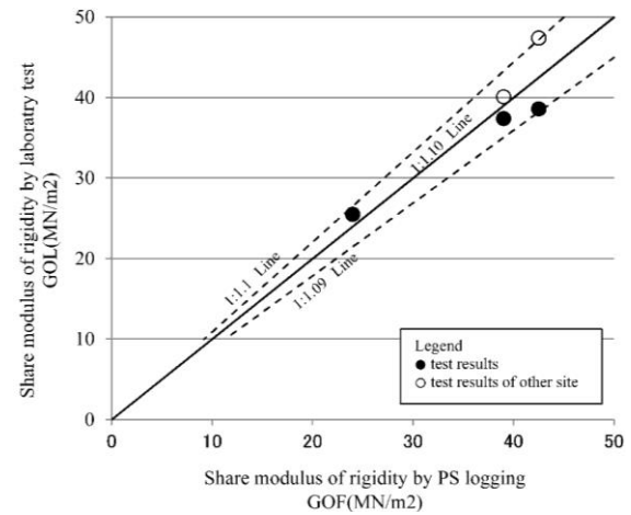
Figure 7. Comparison of shear modulus obtained from laboratory test and PS logging
