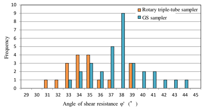
Figure 8. Comparison of angle of shear resistance by sampling method
