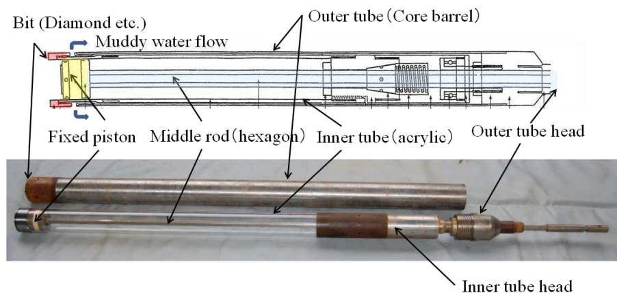
Figure 2. Structure of GS sampler.
