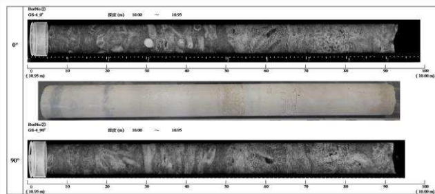
Figure 6. X-ray photograph of undisturbed coral gravel soil (Okinawa Prefecture site)
