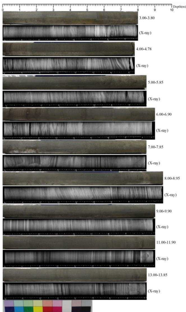
Figure 4. X-ray photograph of undisturbed sandy soil (Chiba Prefecture site)
