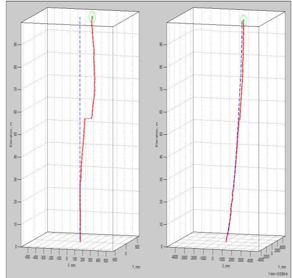
Figure 16. Cumulative displacements, 3D model, west slope Belchatow Field. Figure 17.
