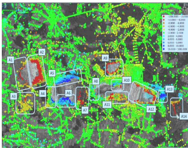
Figure 13. Results of Persistent Scatter Interferometers (PSI).
