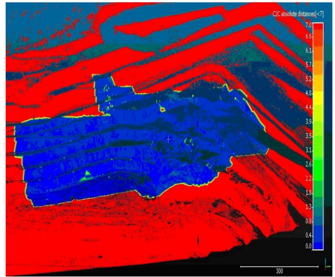
Figure 7. Comparison of LiDAR point cloud and the aerial image after 3-month time, ground movement (Nov 2016–March 2017) west slope of the Belchatow Field, Ineris (France). source: Slopes project report (Marshall et al 2019).
