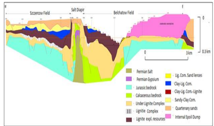
Figure 3. Geological WE cross-section of Belchatow, Szczercow field
