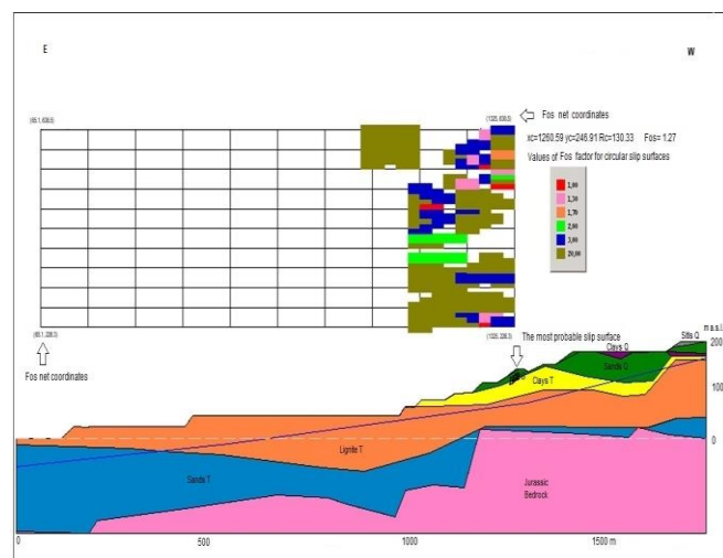
Figure 25. Slope stability analysis, 20WE, LEM Janbu Method, Fos = 1,27.
