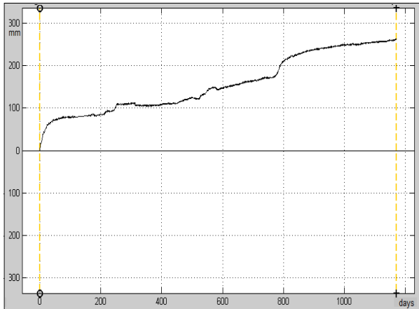
Figure 18. The magnitude of displacement in x and y direction, west slope Belchatow Field.
