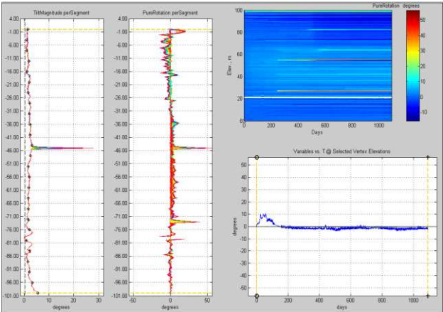
Figure 20. Tilt magnitude and direction control from the magnetometers.
