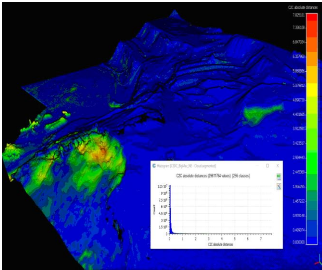
Figure 5. Comparison of LiDAR UAV measurements with aerial photogrammetry, displacement after three months (November 2016–March 2017) west slope of Belchatow Field, Ineris (France). source: Slopes project report Marshall et al 2019.
