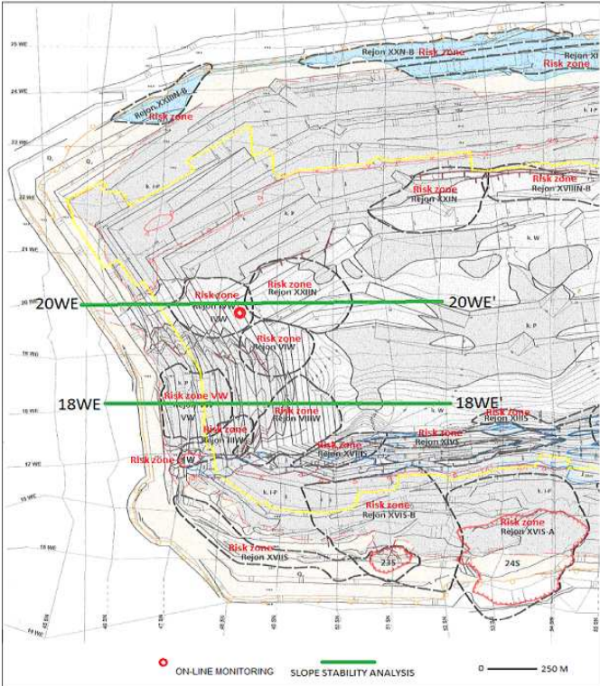
Figure 21. Location of slope stability analysis, risk zones, and monitoring instrumentation.
