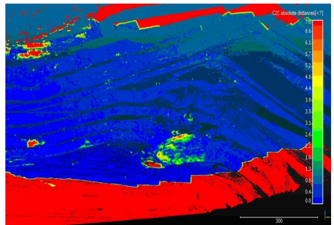
Figure 8. Comparison of TLS terrestrial laser scanning and the aerial photogrammetry (June 2016–March 2017) west slope of Belchatow Field, Ineris (France). source: Slopes project report (Marshall et al 2019).
