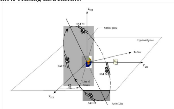
Figure 10. COSMO-SkyMed nominal orbit configuration
