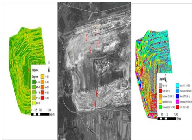
Figure 6. Interpretation of west slope of the Belchatow Field parameters based on TLS laser scanning, University of Exeter (UK) source: Slopes project report (Marshall et al 2019).
