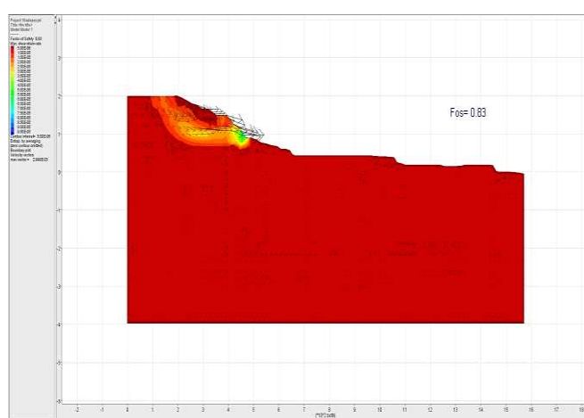
Figure 24. Slope stability analysis, 18 WE, SSR method, 20WE, Fos= 0.83.
