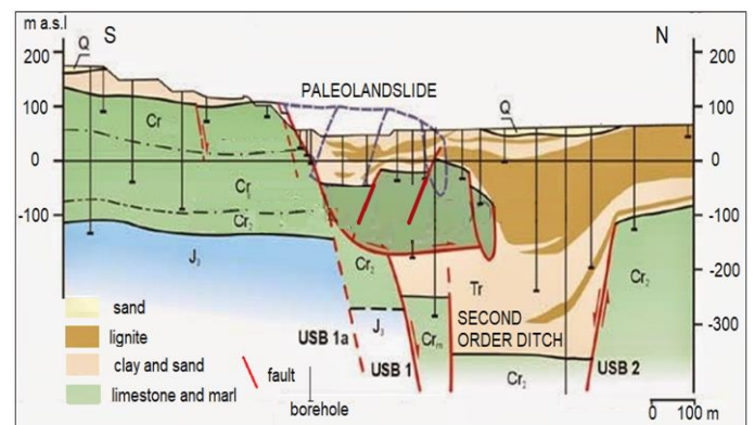
Figure 4. Cross-section of second-order ditch zone (Czarnecki and Felisiak, 2004).
