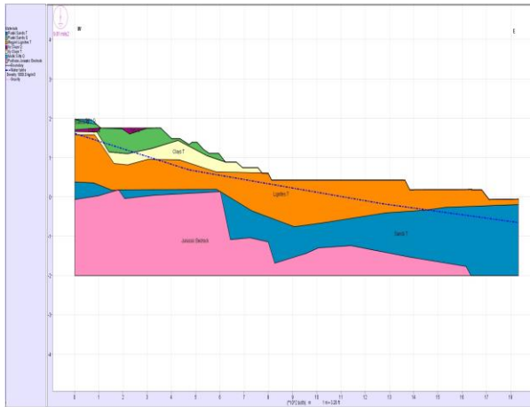
Figure 22. Slope stability analysis 20WE, SSR Method, geotechnical layers.
