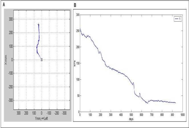
Figure 19. Displacement direction (A) and pore pressure at 30 m depth (B).
