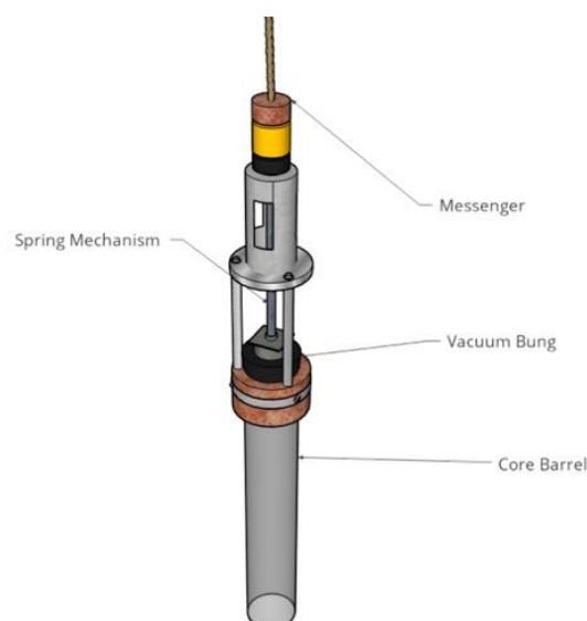
Figure 2. Glew gravity coring device.
