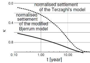
Figure 11. The time dependency of the mechanical type settlement (without biodegradation, see e.g., -Gourc [7])
