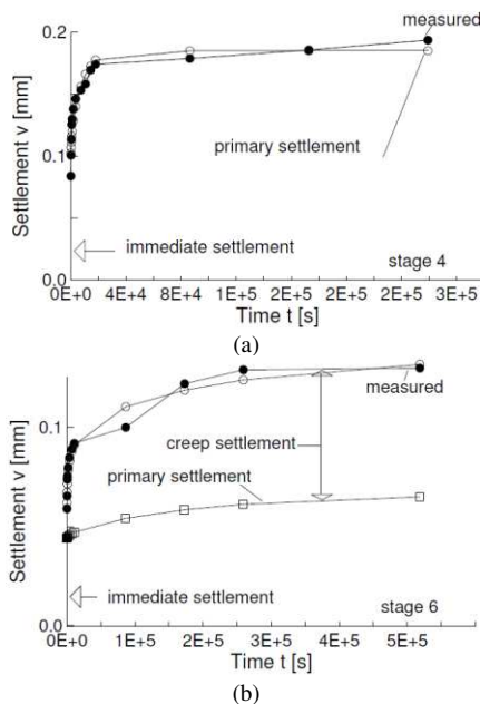
Figure 8. The compression test, sample 3. The variation of the various settlement components with time. (a) Model A, stage 4. (b) Model AC, stage 6.
