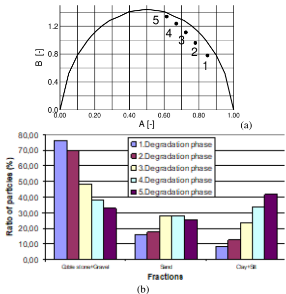
Figure 3. (a) The entropy diagram, the grading curves for degradation phases 1 to 5 (b) Grading curve data (Varga, [36], Table 2)
