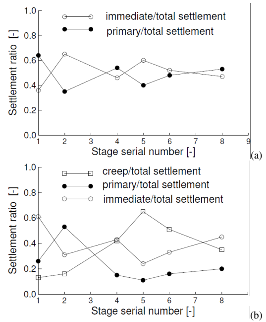
Figure 9. Compression test, sample 3. The settlement components with stage load. (a) Model A (modified Terzaghi's model). (b) Model AC (modified Bjerrum's model)
