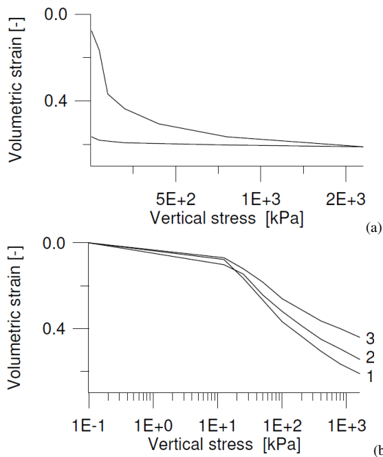
Figure 5. The compression tests. (a) Compression curve of sample 1 with unloading. (b) Compression curves for samples 1 to 3 in log scale
