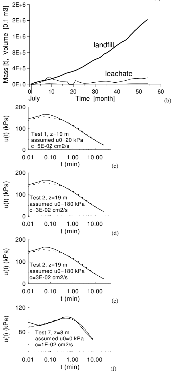
Figure 2. The Pusttazámor landfill site. (a) Site plane of the first phase, (b) Some data of the filling process. (c) to (f) Measured and fitted dissipation curves Figure 7 Measured and fitted dissipation curves (test 1, 2 and 7)
