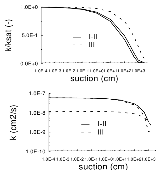
Figure 4. The permeability function of the mineral layers
