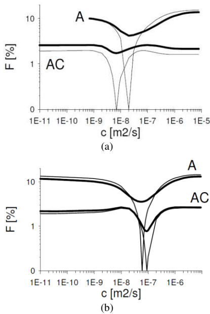
Figure 6. The reliability of the inverse problem solution. The compression test, sample 3, the deepest section of the real-life (thick) and the closest noise-free (thin) merit functions (indicating the uniqueness of the solution and the error of parameter p ) with respect to parameter c . (a) and (b) stage 4 and stage 8, resp. Figure 7.
