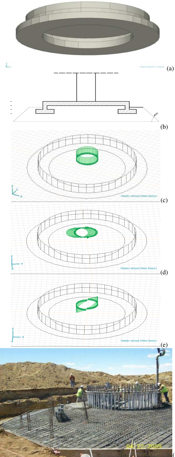
Figure 10. The ring foundation of the turbine tower body. (a) Planned in this work. The connection of the of the turbine tower body: Vertical force (b), horizontal force (c) and moment distribution (d). (f) Constructed in Spadina
