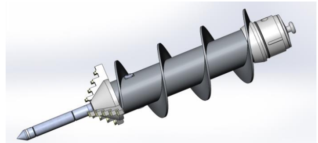
Figure 4. The multi-parameter sensing device
