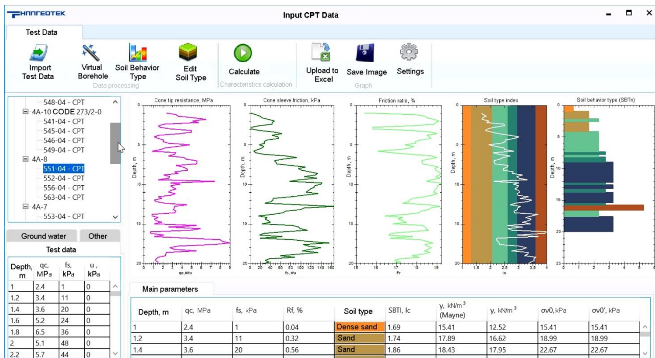
Figure 5. Interpretation of static penetration data
