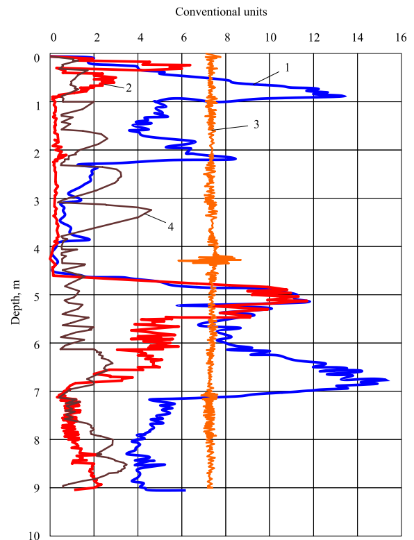
Figure 2. Parameters of sounding: 1 – Torque; 2 – Feed force; 3 – Rotational speed; 4 – Linear speed
