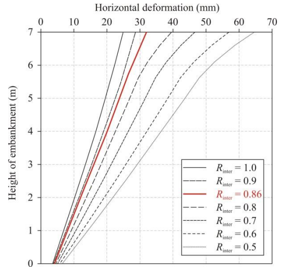
Figure 15. Horizontal deformation of the side of the embankment made of coarse-grained soil, Model 2
