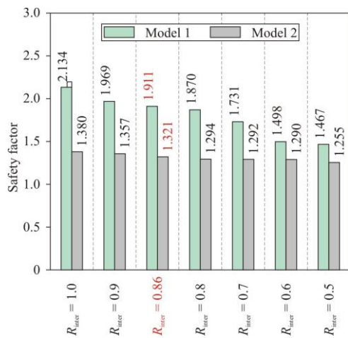
Figure 20. Safety factor for embankments made of coarse-grained soil
