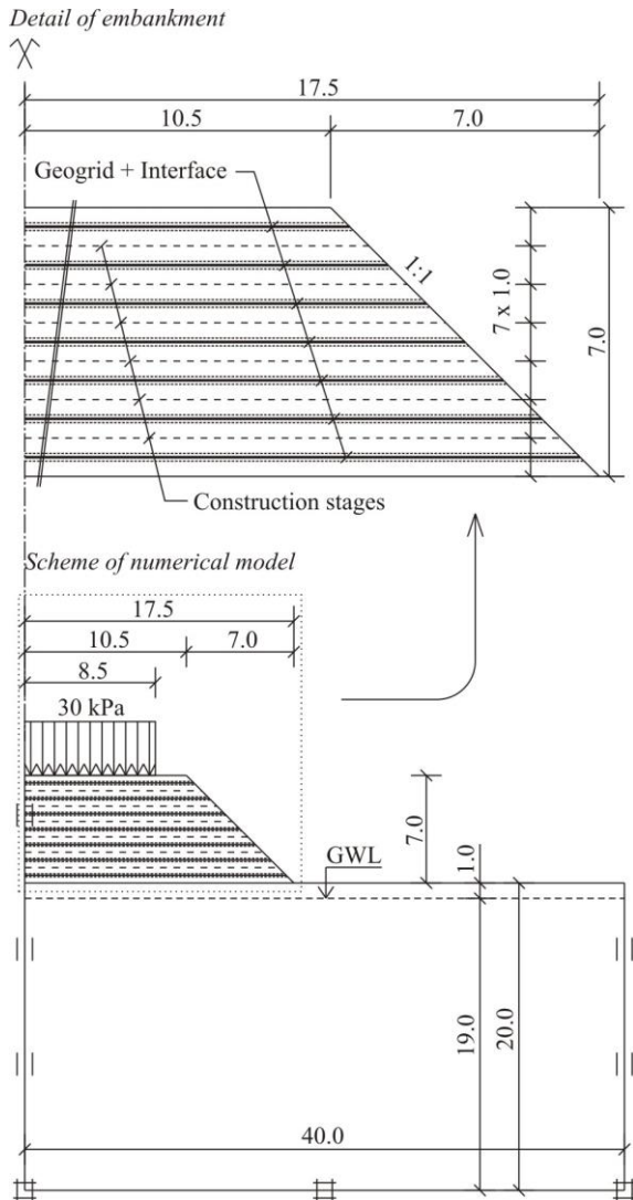
Figure 4. Scheme of Model 1
