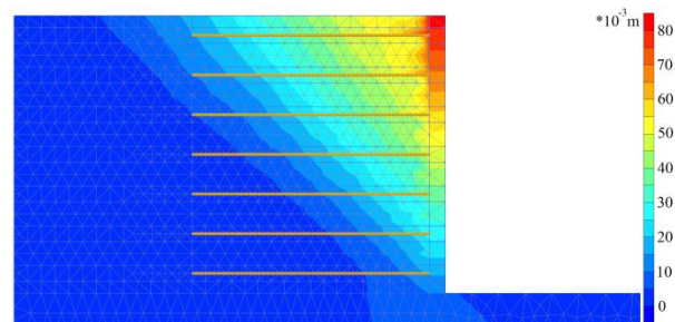
Figure 17. Horizontal deformations of the embankment, Model 2 ( R_{inter} = 0.8 )
