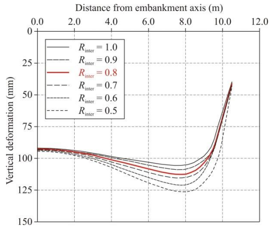
Figure 18. Settlement of the top of the embankment made of fine-grained soil, Model 2
