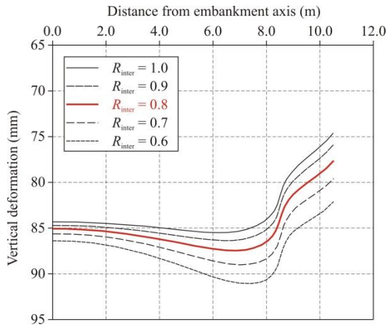
Figure 12. Settlement of the top of the embankment made of fine-grained soil, Model 1
