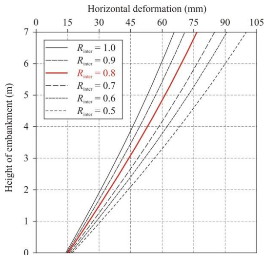
Figure 19. Horizontal deformation of the side of the embankment made of fine-grained soil, Model 2
