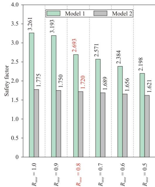
Figure 21. Safety factor for embankments made of fine-grained soil
