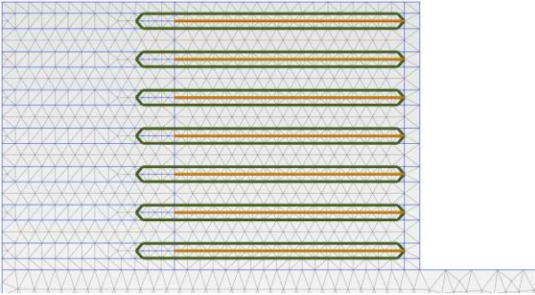
Figure 7. The mesh coarseness of the embankment, Model 2
