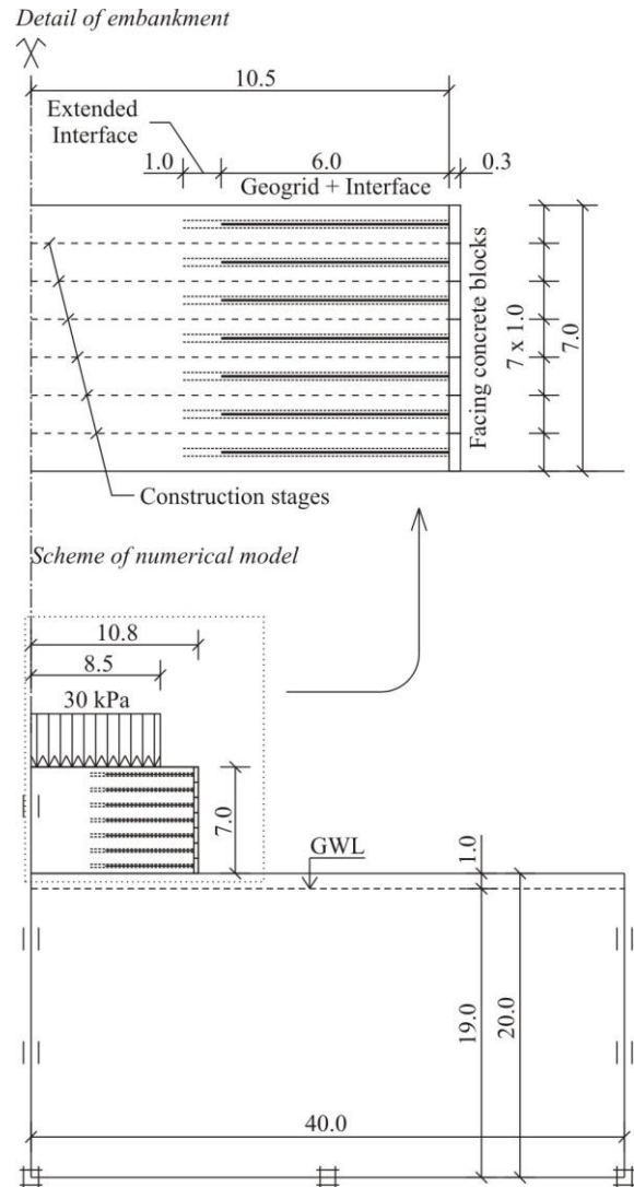
Figure 5. Scheme of Model 2
