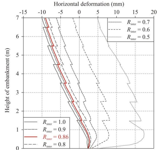
Figure 9. Horizontal deformation of the side of the embankment made of coarse-grained soil, Model 1
