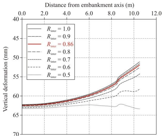
Figure 8. Settlement of top of the embankment made of coarse-grained soil, Model 1
