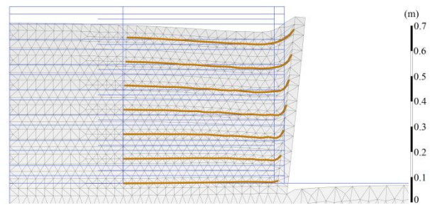
Figure 16. Deformed model of the embankment, Model 2 ( R_{inter} = 0.8 )
