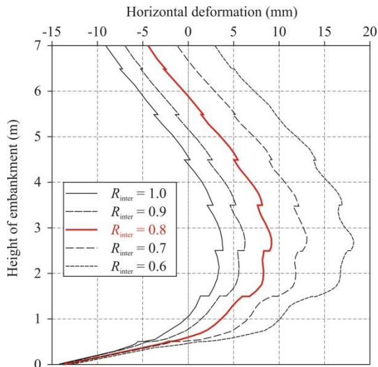
Figure 13. Horizontal deformation of the side of the embankment made of fine-grained soil, Model 1
