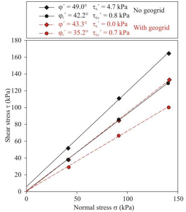
Figure 3. Results of the shear tests of coarse-grained soil sample
