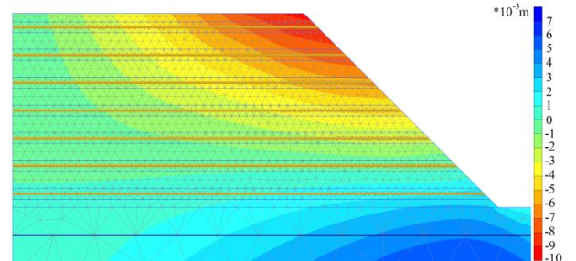
Figure 11. Horizontal deformations of the embankment, Model 1 ( R_{inter} = 0.86 )
