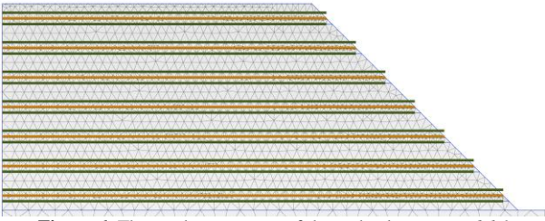
Figure 6. The mesh coarseness of the embankment, Model 1
