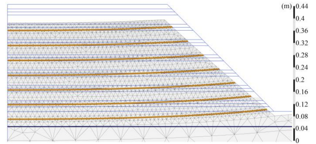
Figure 10. Deformed model of the embankment, Model 1 ( R_{inter} = 0.86 )
