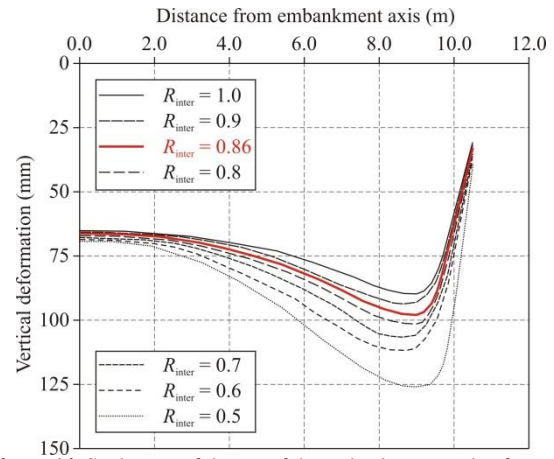
Figure 14. Settlement of the top of the embankment made of coarse-grained soil, Model 2
