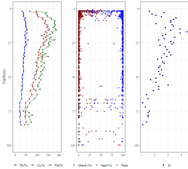
Fig 5. Average index properties
