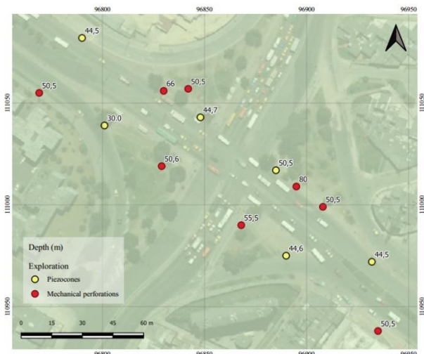
Fig 4. Site Investigation location plan - Site 3
