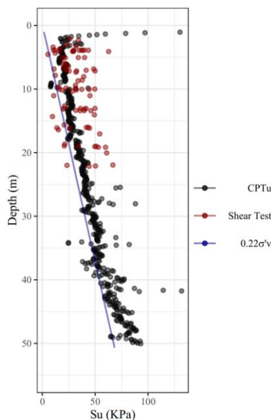
Fig 9. Su obtained for Zone 2 CPTu
