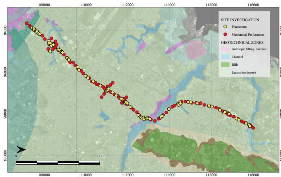
Fig 2. Geotechnical site investigation location plan
