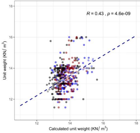
Fig 6. Soil unit weight obtained from qt and fs
