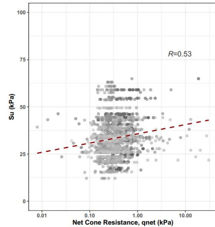
Fig 8. S_u and net tip resistance
