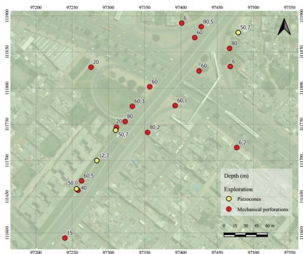
Fig 3. Site Investigation location plan - Site 2
