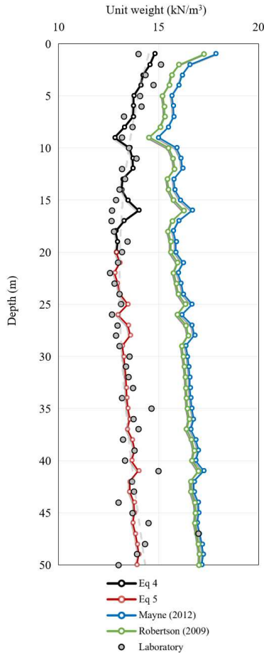
Fig 7. Unit weight measured in laboratory tests and calculated using correlations.
