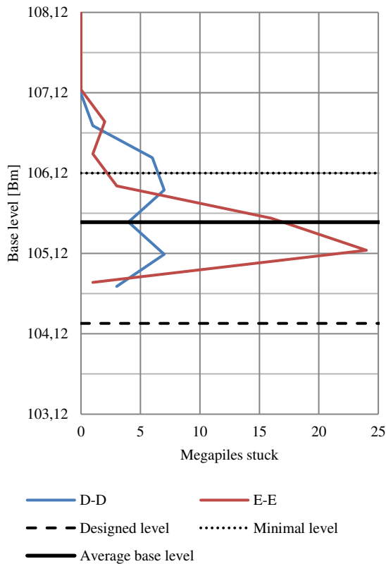
Figure 8. Reached base levels of the constructed piles
