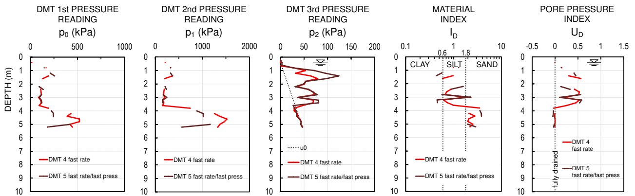
Figure 6. Effect of variable pressurization rate on Medusa DMT results (fast penetration rate).
