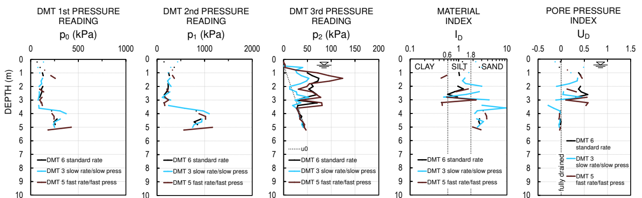
Figure 7. Combined effects of variable penetration rate and variable pressurization rate on Medusa DMT results.
