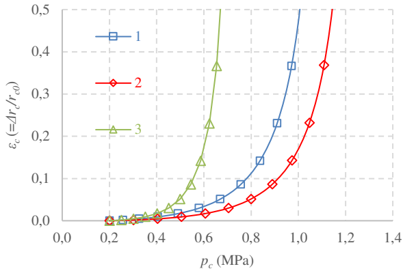
Figure 5. Theoretical p - \epsilon_c curves1
