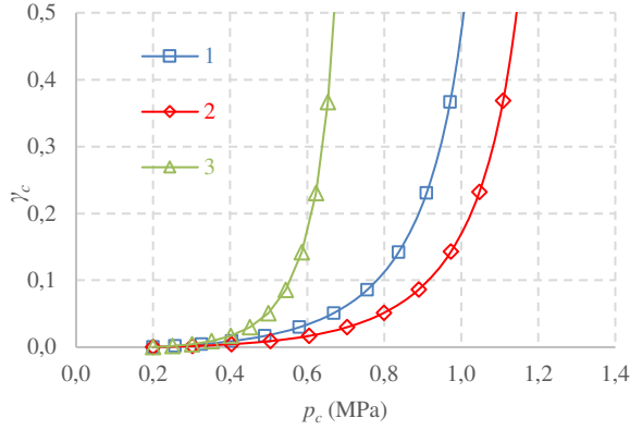
Figure 3. Theoretical p_c - \gamma_c curves
