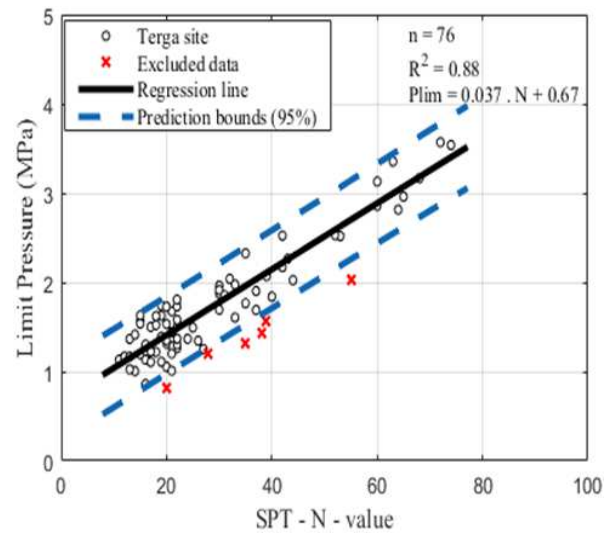
Figure 11. Relationship between limit pressure and SPT, N-value for sand of Terga site
