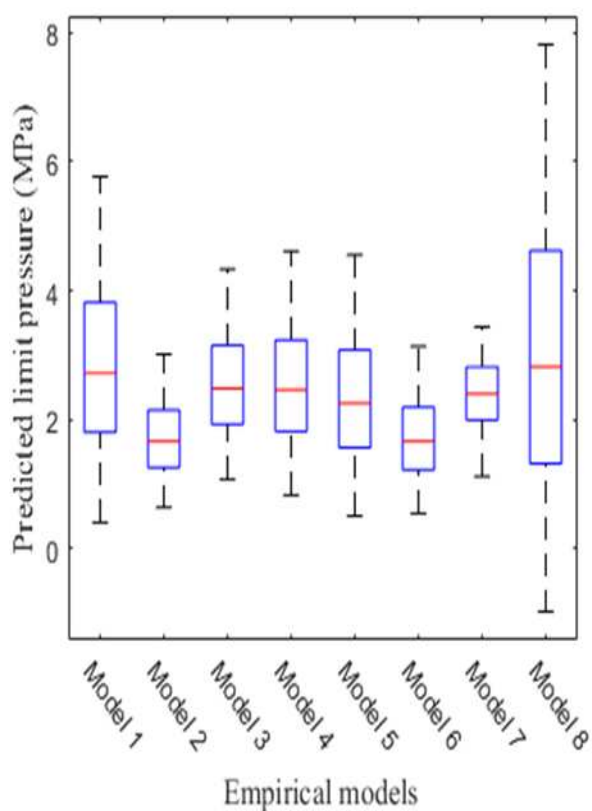
Figure 15. Box plot of the predicted limit pressure for some correlation of literature and correlation of this study
