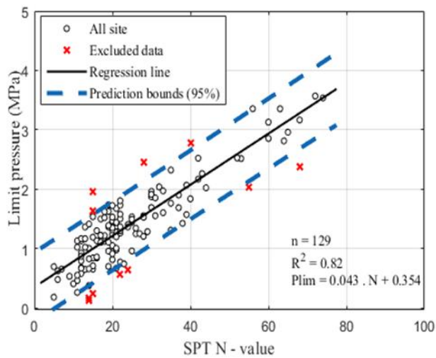
Figure 13. Relationship between limit pressure and SPT, N-value for sand of all sites
