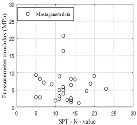
Figure 8. Relationship between pressuremeter modulus and SPT, N-value for sand of Mostaganem site
