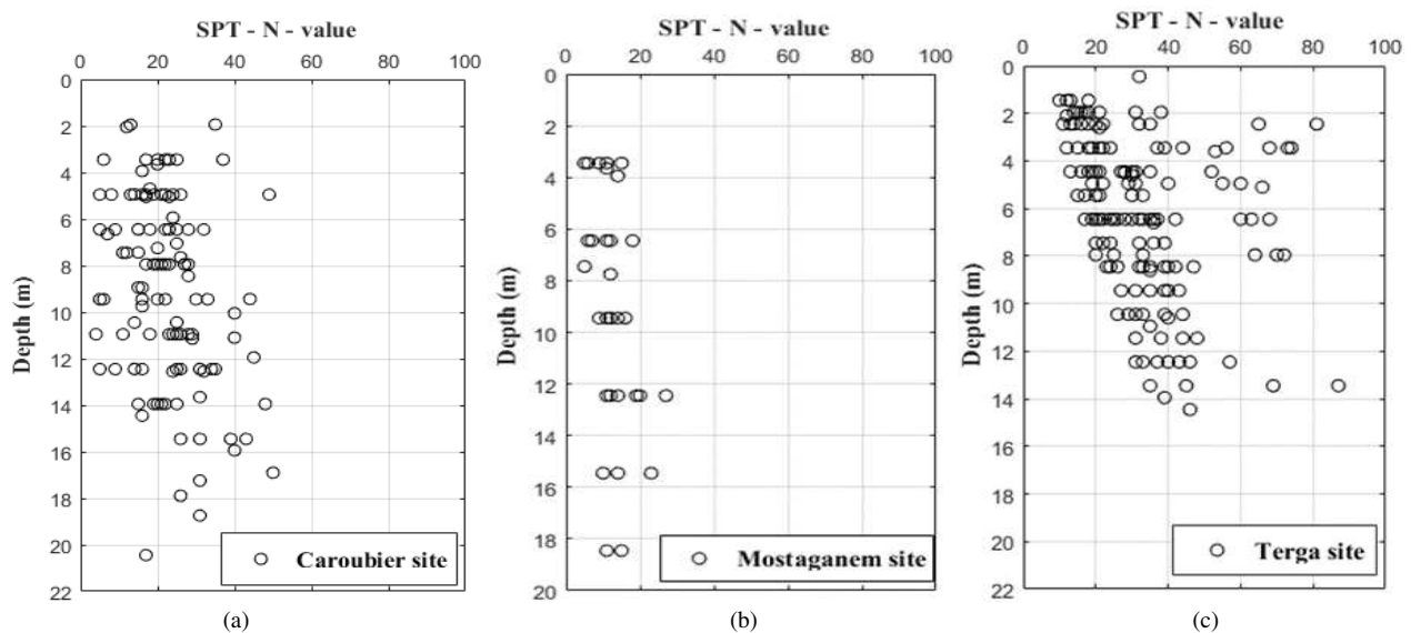
Figure 1. Profile of SPT, N-value for sites: (a) Caroubier, (b) Mostaganem, (c) Terga.
