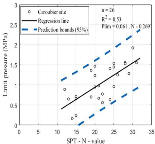
Figure 9. Relationship between limit pressure and SPT, N-value for sand of Caroubier site
