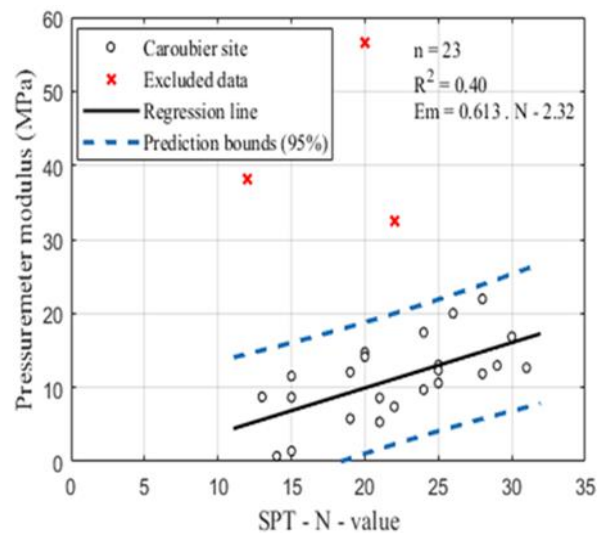
Figure 10. Relationship between pressuremeter modulus and SPT, N-value for sand of Caroubier site
