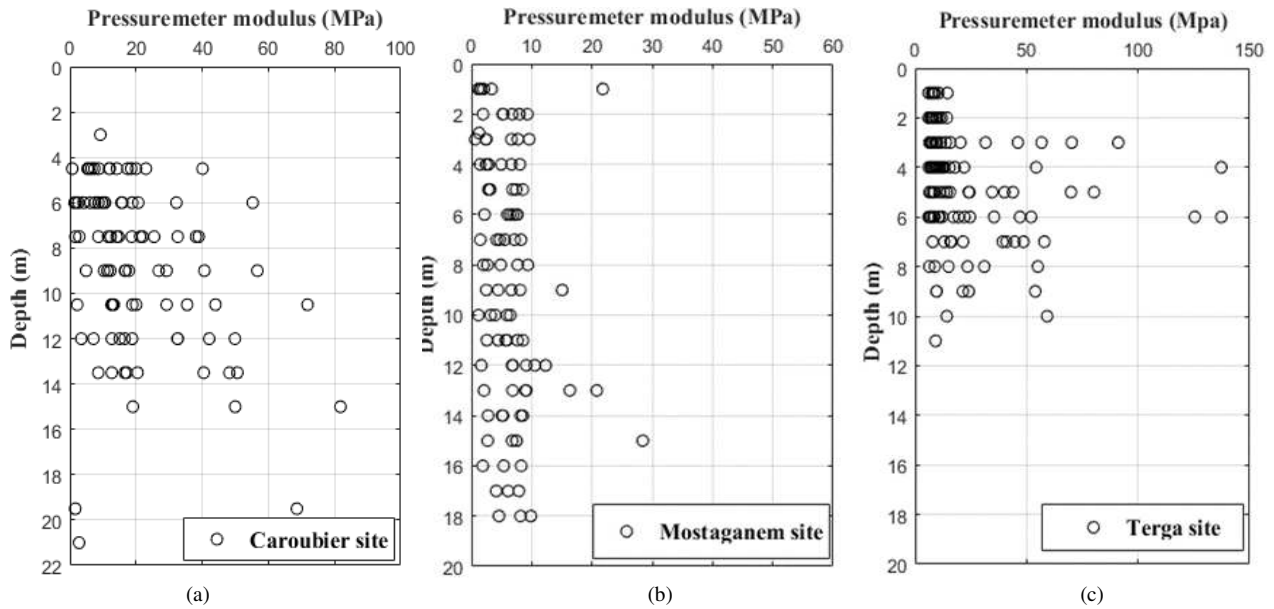
Figure 3. Profile of pressuremeter modulus for sites: (a) Caroubier, (b) Mostaganem, (c) Terga
