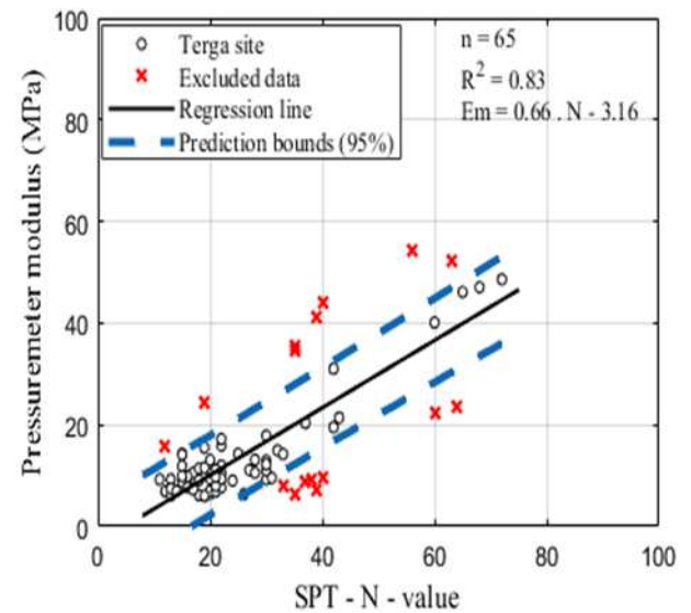
Figure 12. Relationship between pressuremeter modulus and SPT, N-value for sand of Terga site
