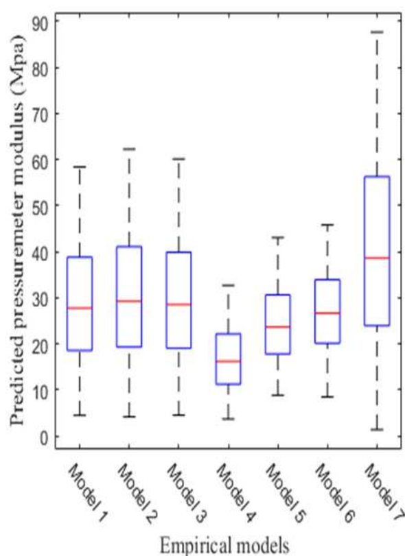
Figure 16. Box plot of the predicted pressuremeter modulus for some correlation of literature and correlation of this study.
