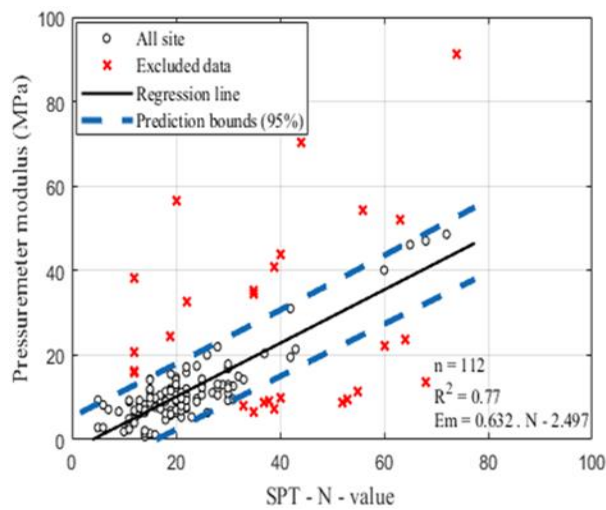
Figure 14. Relationship between pressuremeter modulus and SPT, N-value for sand of all sites
