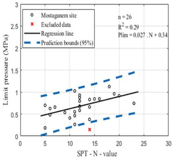
Figure 7. Relationship between limit pressure and SPT, N-value for sand of Mostaganem site
