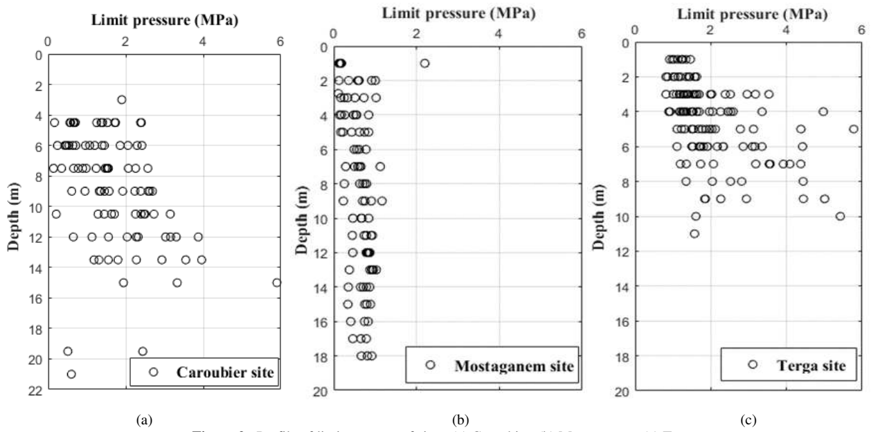
Figure 2. Profile of limit pressure of sites: (a) Caroubier, (b) Mostaganem, (c) Terga.
