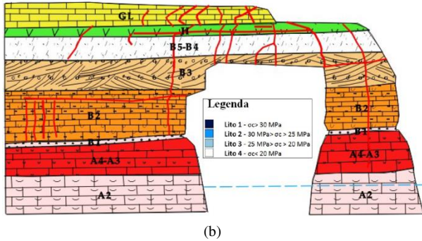
Figure 11. (a) Wied il-Mielah (Maltese Islands); (b) engineering geological model.
