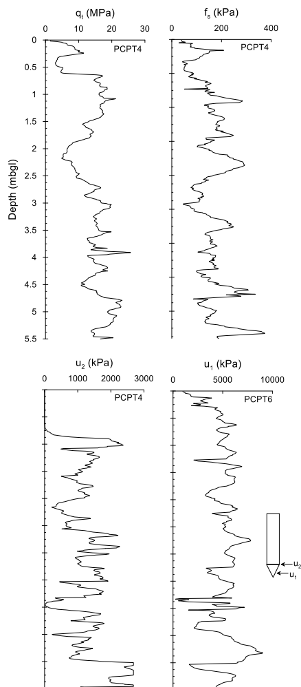
Figure 1. Typical profiles of cone resistance, q_t , sleeve friction, f_s , pore pressure at the sleeve position, u_2 and u_1 measured in PCPT4 at the Imperial College test site: Note u_1 plot is from an adjacent CPT [16]
