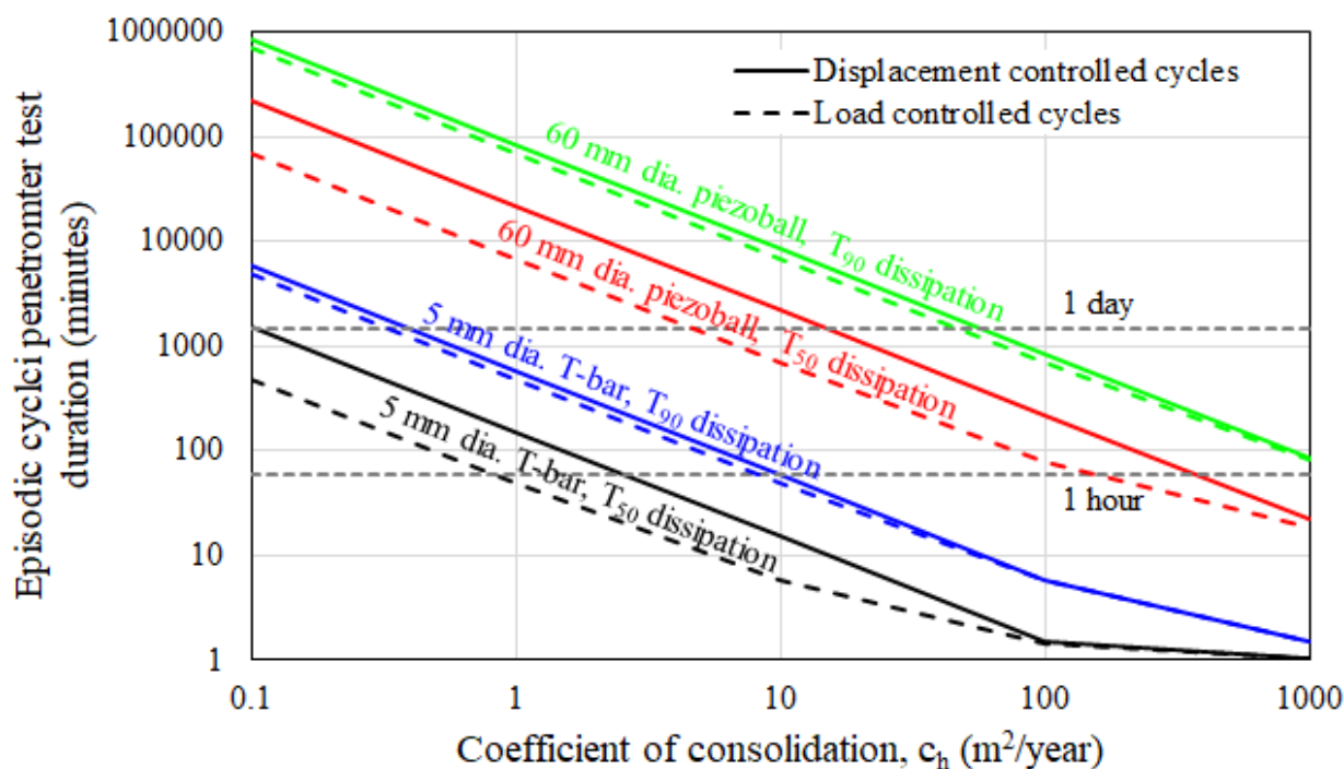
Figure 18. Estimated durations of episodic cyclic penetrometer tests assuming a rigidity index, I_r = 100 .
