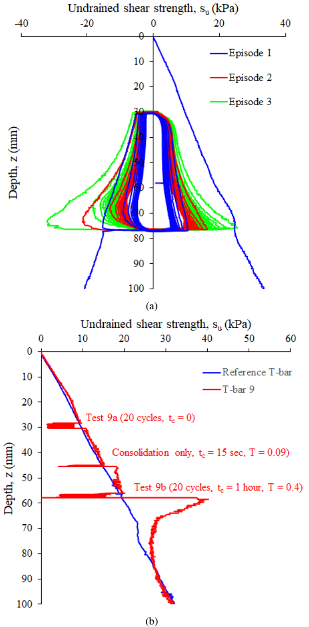
Figure 16. Changes in soil strength from: (a) displacement-controlled cycles (Type II); (b) load-controlled cycles (Type III).
