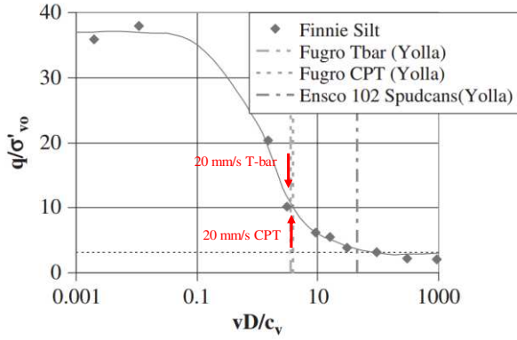
Figure 6. Partial drainage during T-bar and CPT tests at Yolla (after Erbrich, 2005).
