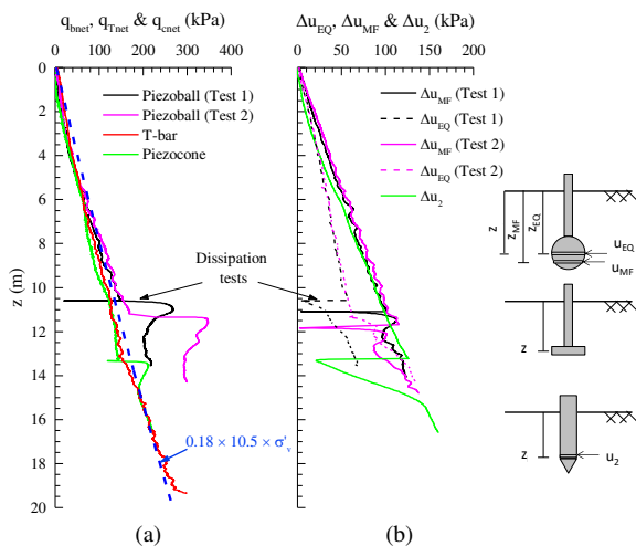
Figure 2. Penetration profiles from centrifuge tests in normally consolidated kaolin clay: (a) net penetration resistance for piezoball, T-bar and piezocone; (b) excess pore pressure for piezoball mid-face and equator and piezocone u_2 measurement locations.
