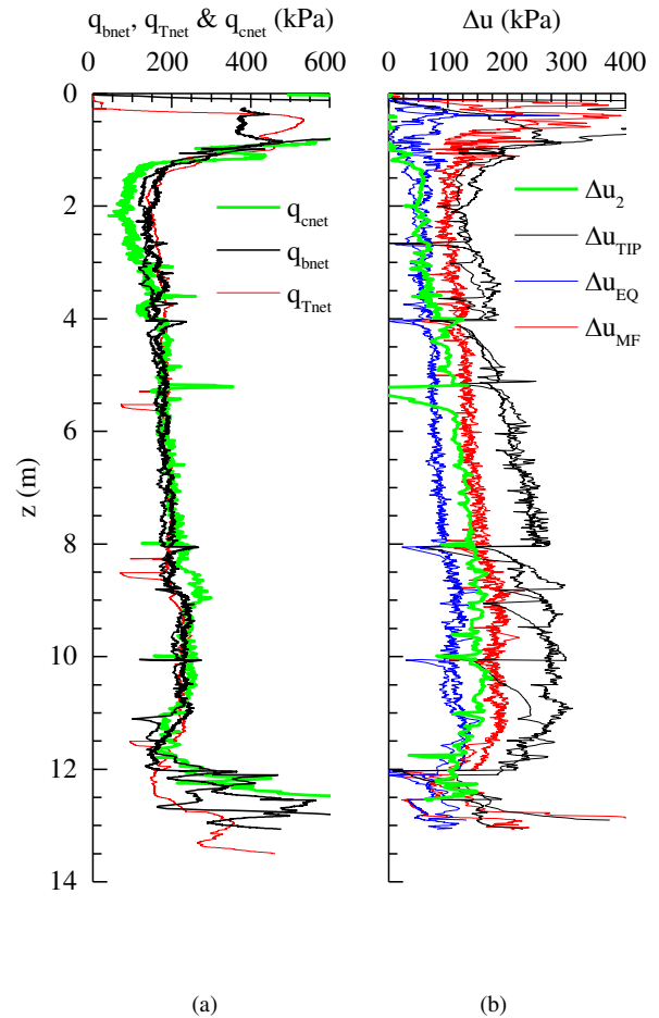
Figure 3. Penetration profiles from field tests in Ballina clay: (a) net penetration resistance for piezoball, T-bar and piezocone; (b) excess pore pressure for piezoball tip, mid-face and equator and piezocone u_2 measurement locations.
