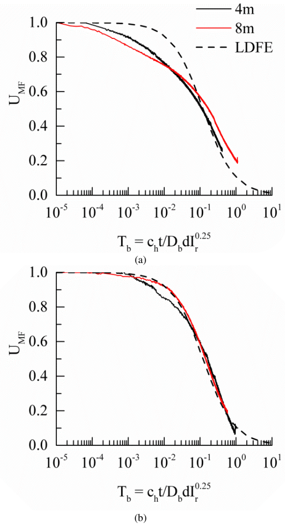
Figure 11. Measured and numerical piezoball excess pore pressure dissipation responses after penetration at: (a) 20 mm/s, (b) 0.02 mm/s.
