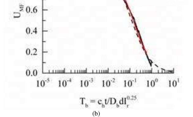
Figure 10. Comparison between Ballina field piezoball dissipation responses and the theoretical solution: (a) equator, (b) mid-face.
