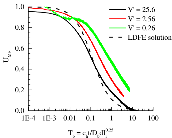
Figure 12. Non-dimensional piezoball dissipation profiles for the piezoball mid-face measurement location following undrained and partially drained penetration.
