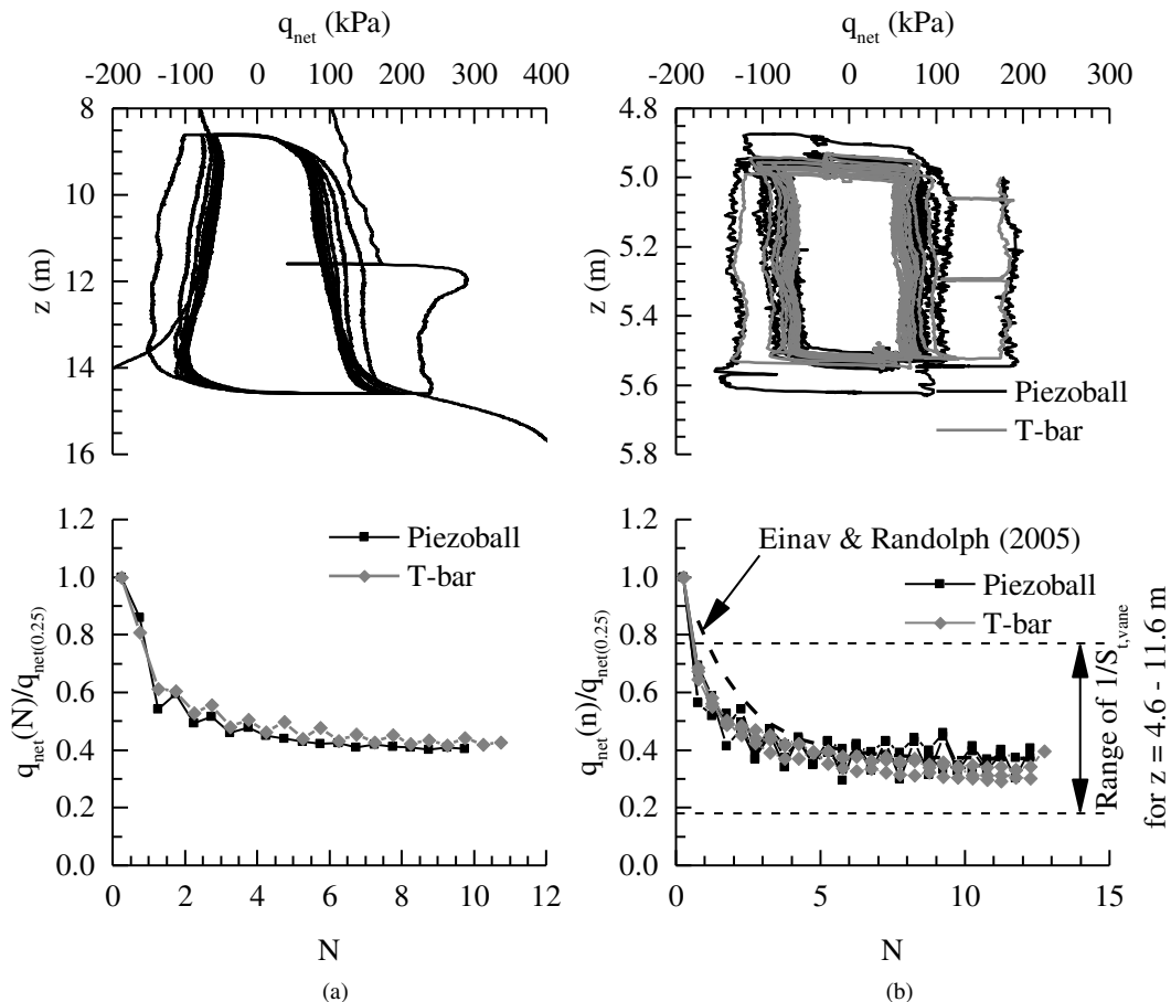
Figure 4. Piezoball and T-bar cyclic remoulding response: (a) centrifuge tests in kaolin clay; (b) field tests in Ballina clay.
