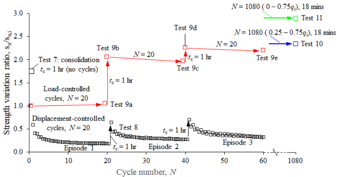
Figure 17. Comparison of changing soil strength due to load and displacement controlled loading cycles in centrifuge penetrometer tests in a reconstituted normally consolidated carbonate silt.
