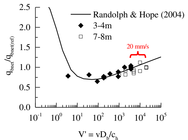
Figure 5. Piezoball backbone curves of net penetration resistance
