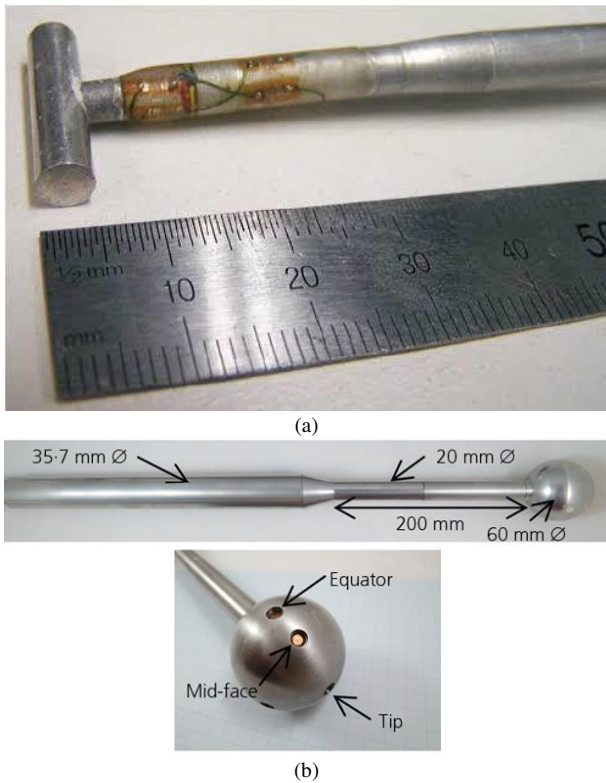
Figure 1. Full-flow penetrometers: (a) T-bar (centrifuge scale); (b) piezoball (field scale).
