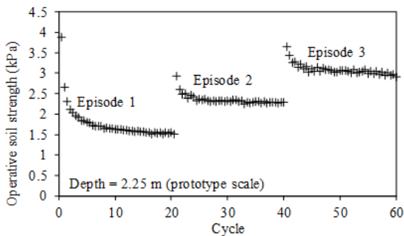
Figure 14. Changes in strength during episodic cyclic T-bar test in kaolin clay (after Hodder et al. 2009).
