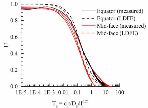
Figure 9. Piezoball dissipation response in kaolin clay compared with the numerical (LDFE) solution
