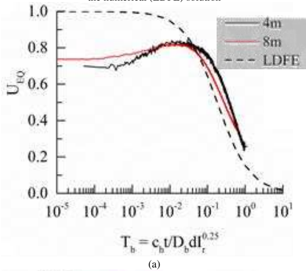
Figure 9. Piezoball dissipation response in kaolin clay compared with the numerical (LDFE) solution
