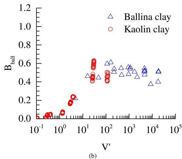
Figure 13. B_{ball} as a partial consolidation indicator: (a) mid-face (b) equator.
