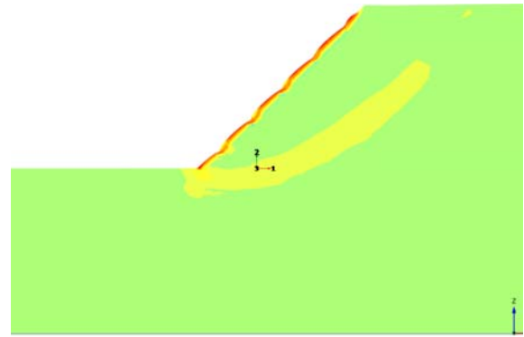
Figure 9. Incremental shear strains of the numerical simulations of the slope stabilization system with a cohesion of 5 \text{ kN/m}^2 in cross-section 1.
