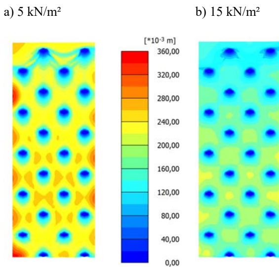
Figure 8. Surface deformation of the numerical simulations with a cohesion of 5 \text{ kN/m}^2 (a) and a cohesion of 15 \text{ kN/m}^2 (b).
