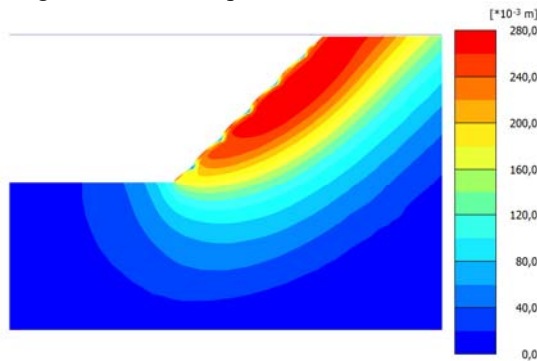
Figure 7. Total displacement of the numerical simulations of the slope stabilization system with a cohesion of 5 \text{ kN/m}^2 in cross-section 1.
