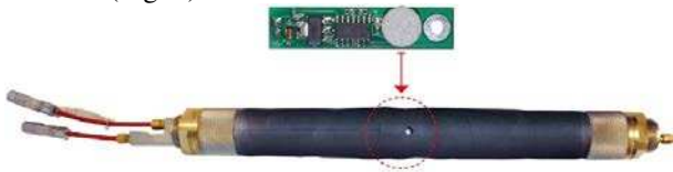
Figure 4. Electronic card with integrated sensor for pore pressure measurement and its place on the sheath (SA Jean Lutz®)
