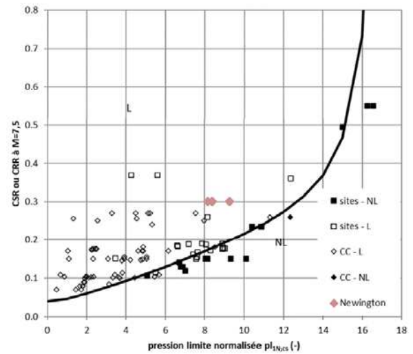
Figure 6. Newington cyclic and monotone tests on the CSR versus normalized p_{LM} diagram
