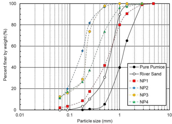
Figure 7. Original particle size distribution curves of the materials tested
