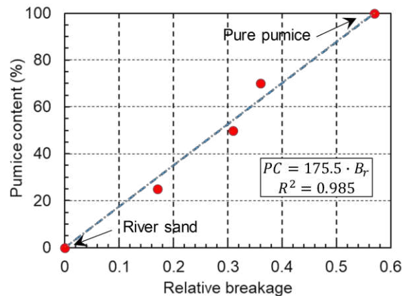
Figure 12. Estimation of pumice content according to the relative breakage
