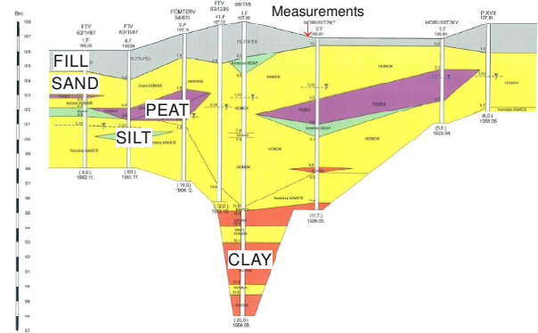
Figure 2. Geological profile [15] at the location of surface wave measurements carried out in Városliget
