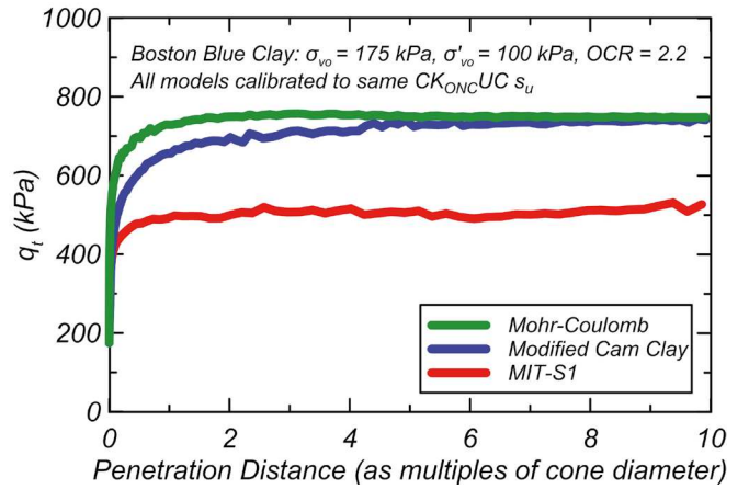
Figure 8. Simulated tip resistance versus penetration distance from wished in-place initial condition (after Moug et al. 2016)
