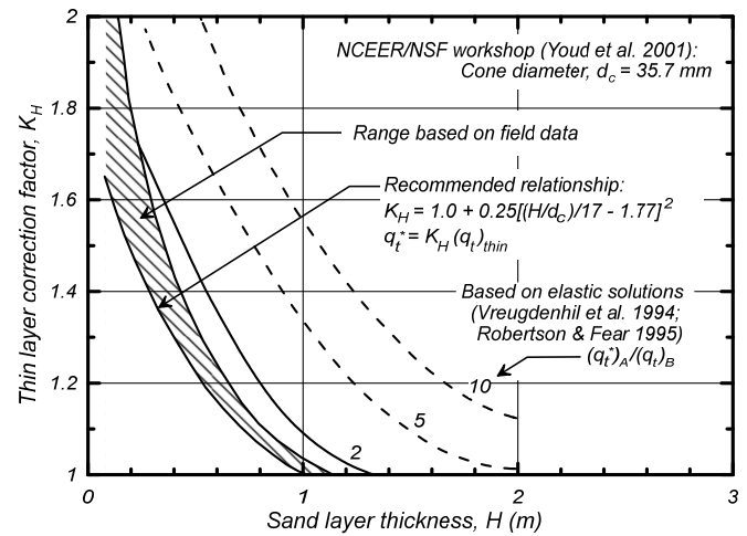
Figure 2. Thin layer correction factors for determining equivalent thick-layer cone tip resistance (modified from Youd et al. 2001; after Idriss and Boulanger 2008)
