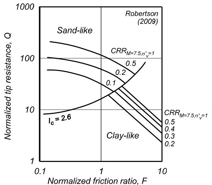
Figure 4. Contours of CRR_{M=7.5, \sigma'_v=1} for sand-like and clay-like soils based on the procedures by Robertson and Wride (1998) for sand-like soils and by Boulanger and Idriss (2007) for clay-like soils (after Robertson 2009)
