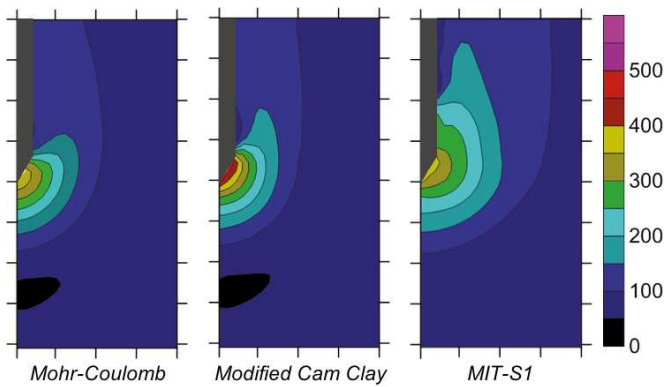
Figure 10. Pore water pressure at 25 cone diameters of penetration in Boston Blue Clay; u_o = 75 kPa prior to penetration (after Moug et al. 2016)
