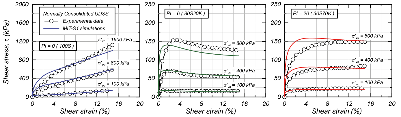
Figure 13. Simulation of undrained monotonic DSS responses for normally consolidated, slurry sedimented specimens of the PI = 0, 6, and 20 soils at different initial consolidation stresses (Price et al. 2015)
