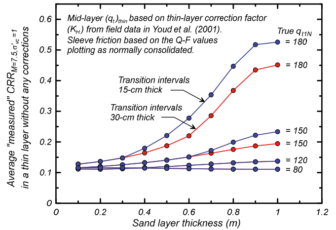
Figure 3. Idealized example illustrating the underestimation of CRR for a thin sand layer embedded between clay layers if transition and thin-layer corrections are not applied
