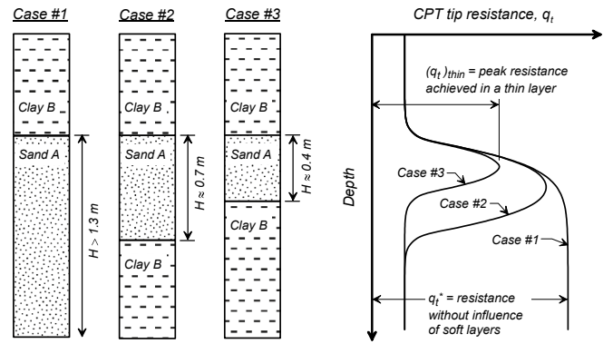
Figure 1. Influence of clay-sand interfaces and sand layer thickness on cone penetration resistance (modified from Robertson and Fear 1995; after Idriss and Boulanger 2008)
