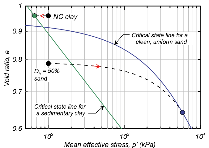
Figure 5. Schematic of loading paths near a penetrating cone in normally consolidated clay (an undrained path) or medium dense sand (a drained path)
