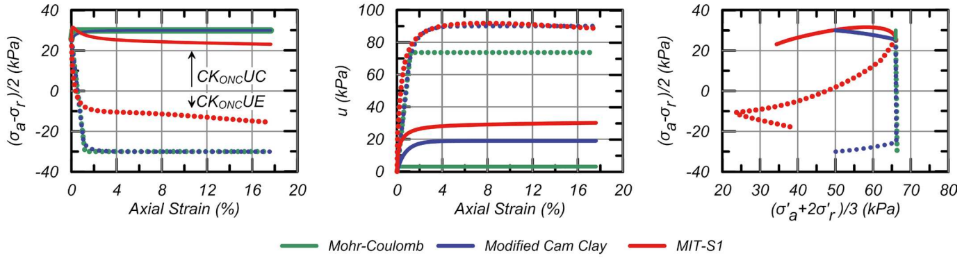
Figure 7. Single element simulations of BBC response in CK_{ONCUC} and CK_{ONCUE} loading using the MC, MCC and MIT-S1 constitutive models calibrated to the same CK_{ONCUC} strength (after Moug et al. 2016)
