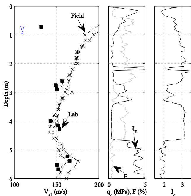
Figure 3: Comparison of lab and field shear wave velocities for samples obtained at Gainsborough Reserve
