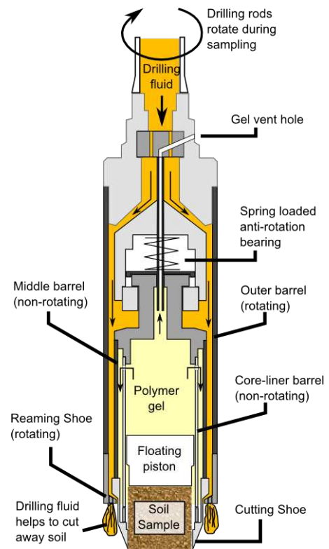
Figure 2: Schematic of GP-TR type sampler
