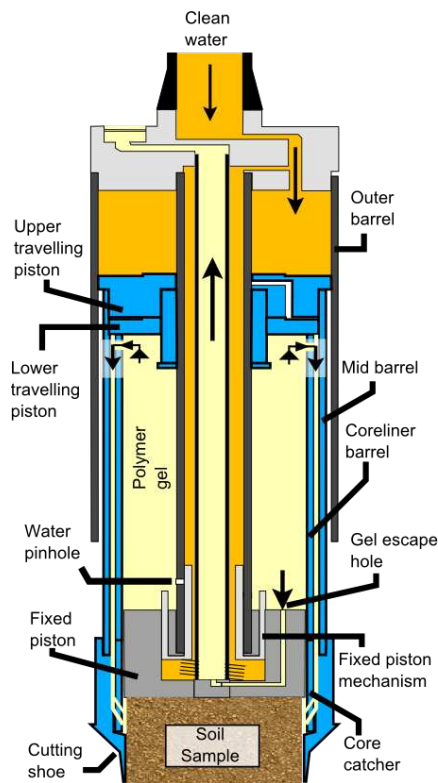
Figure 1: Schematic of GP-S type sampler
