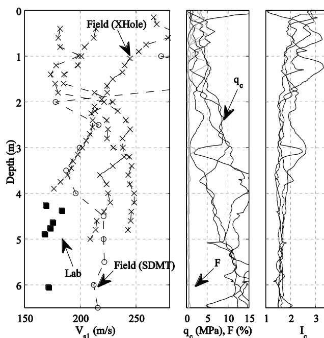
Figure 5: Comparison of lab and field shear wave velocities for samples obtained at Bexley
