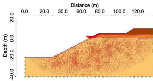
Figure 11 – PLAXIS-analysis
