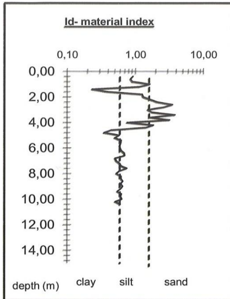
Figure 1. I_D (DMT1)
