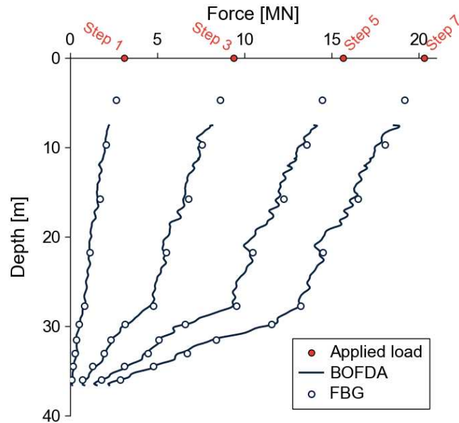
Figure 3. Fibre optic measurements during a load test on a cast-in-situ pile (850 mm diameter)
