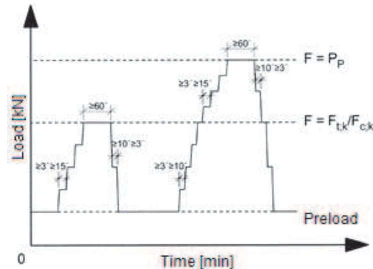
Fig. 6: Test procedure of a pile load test, DGGT (2012)
