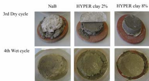
Figure 2. Specimens at the end of the third dry cycle and at the end of the fourth wet cycle
