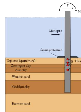
Figure 2. Layout of instrumented monopile, soil stratigraphy and loading on the monopile.
