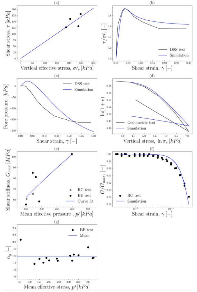
Figure 5. Calibration of clay hypoplasticity parameters for the zomergel layer
