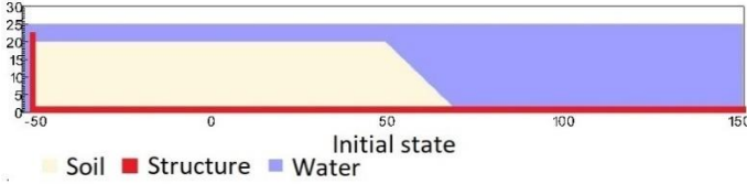
Figure 1. Geometry of the base case slope
