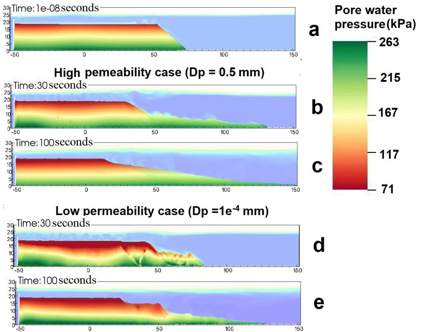
Figure 6. Pore water pressure development for high permeability and low permeability cases
